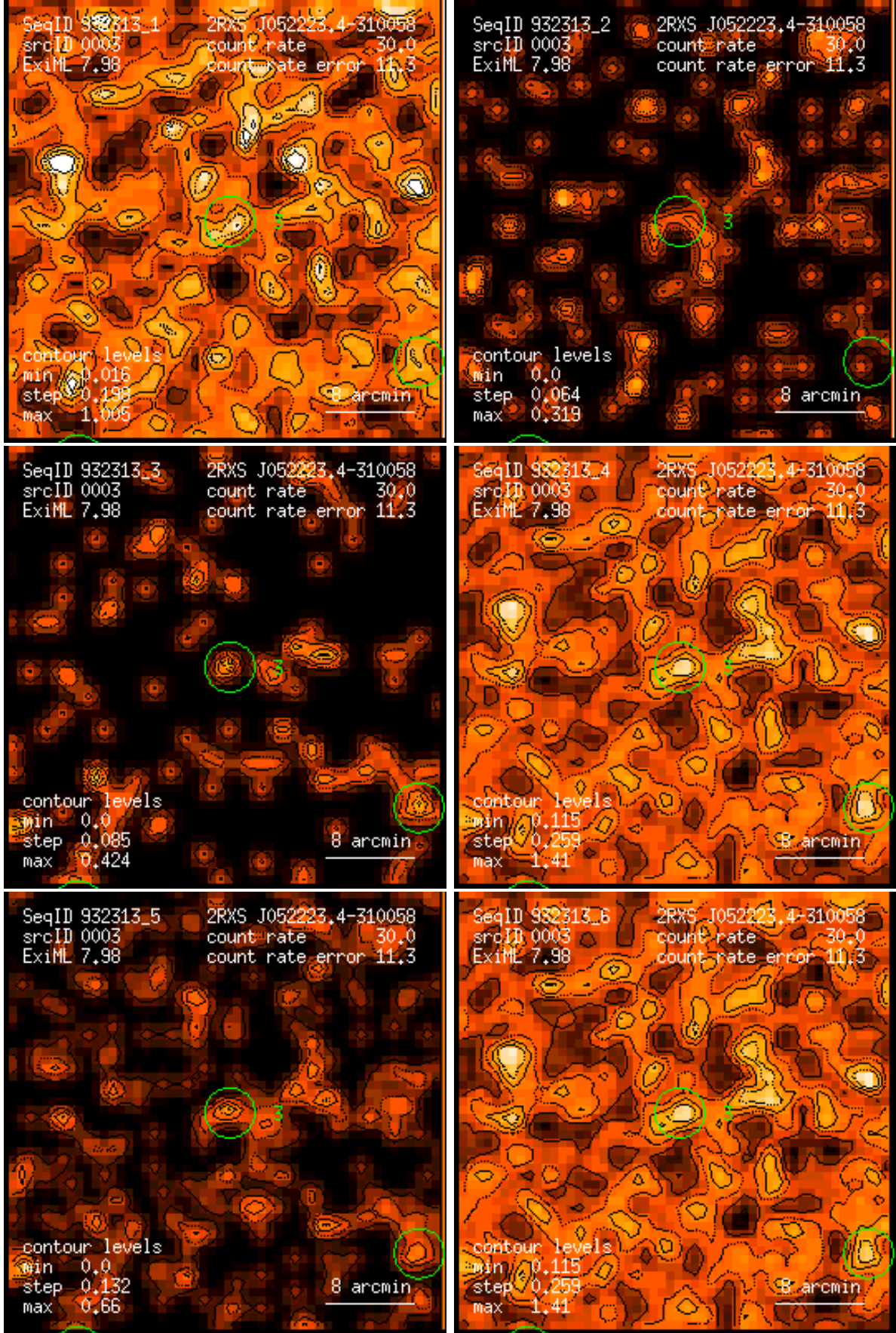
Figure 3: RASS 932313: detection 0003: band rate images, Gaussian filter: (1) PSPC channels 11 – 41, (2) 52 – 90, (3) 91 – 201, (4) 11 – 235, (5) 52 – 201, (6) 11 – 201. Broad band rates in counts/ks. Band rate contour levels in counts/ks/arcmin 2 .
