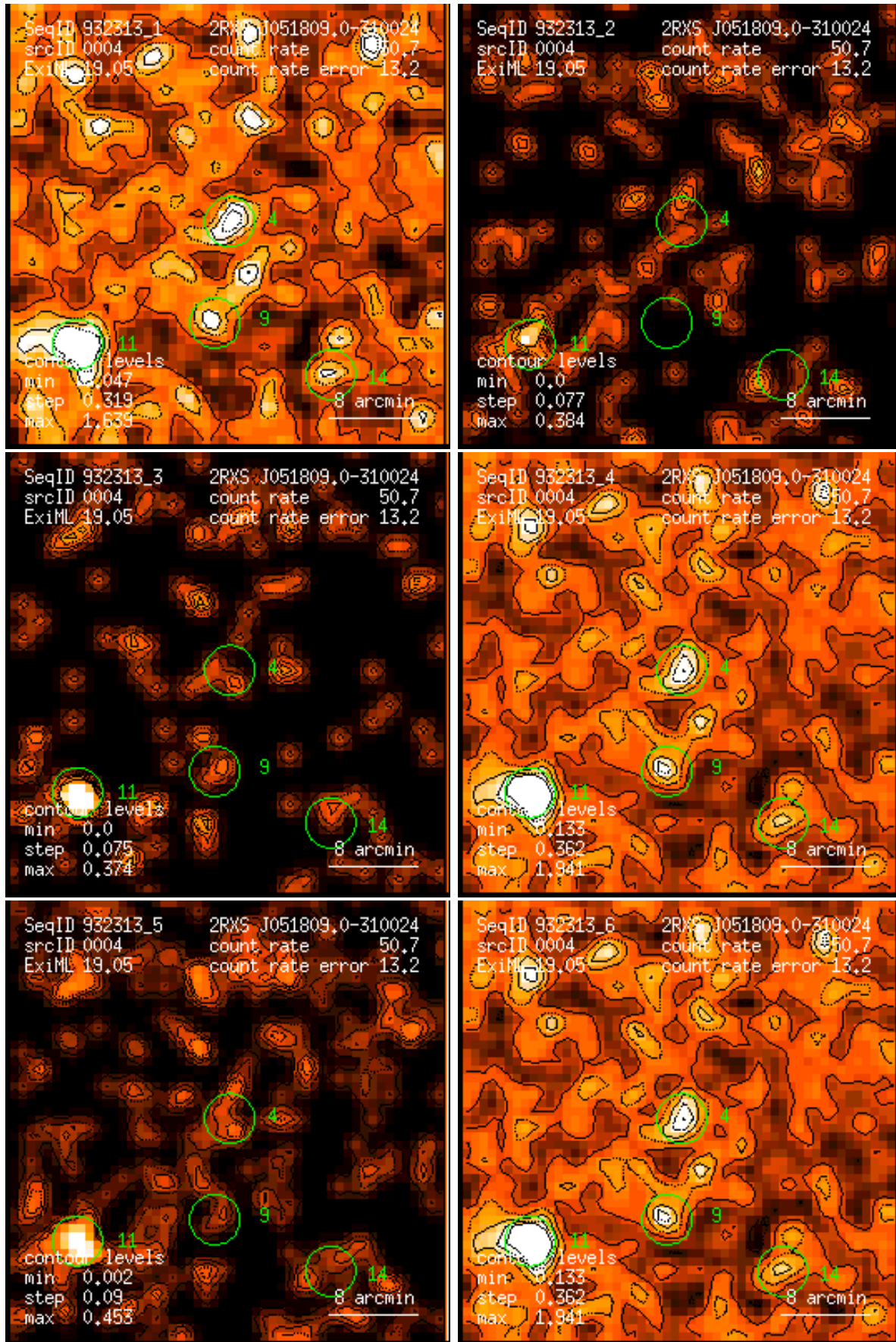
Figure 4: RASS 932313: detection 0004: band rate images, Gaussian filter: (1) PSPC channels 11 – 41, (2) 52 – 90, (3) 91 – 201, (4) 11 – 235, (5) 52 – 201, (6) 11 – 201. Broad band rates in counts/ks. Band rate contour levels in counts/ks/arcmin 2 .
