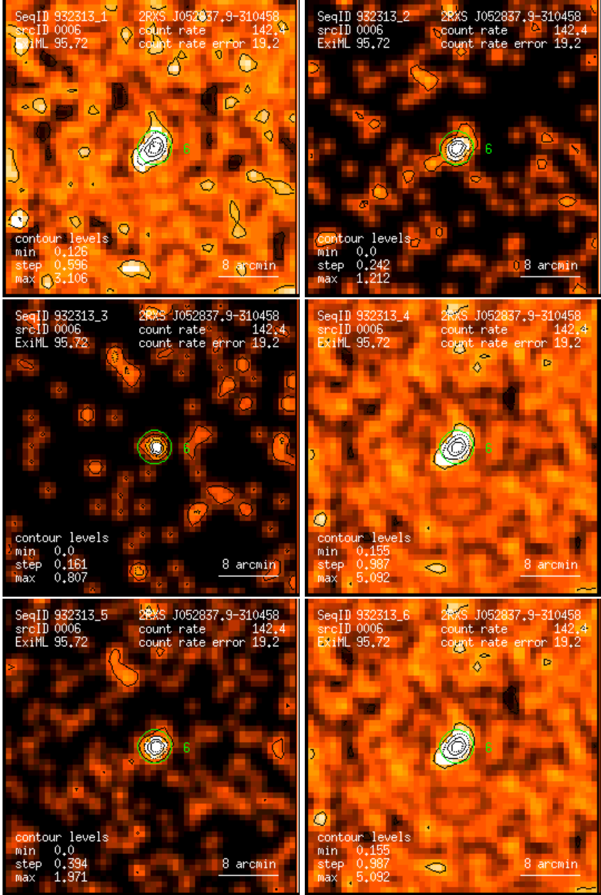
Figure 6: RASS 932313: detection 0006: band rate images, Gaussian filter: (1) PSPC channels 11 – 41, (2) 52 – 90, (3) 91 – 201, (4) 11 – 235, (5) 52 – 201, (6) 11 – 201. Broad band rates in counts/ks. Band rate contour levels in counts/ks/arcmin 2 .
