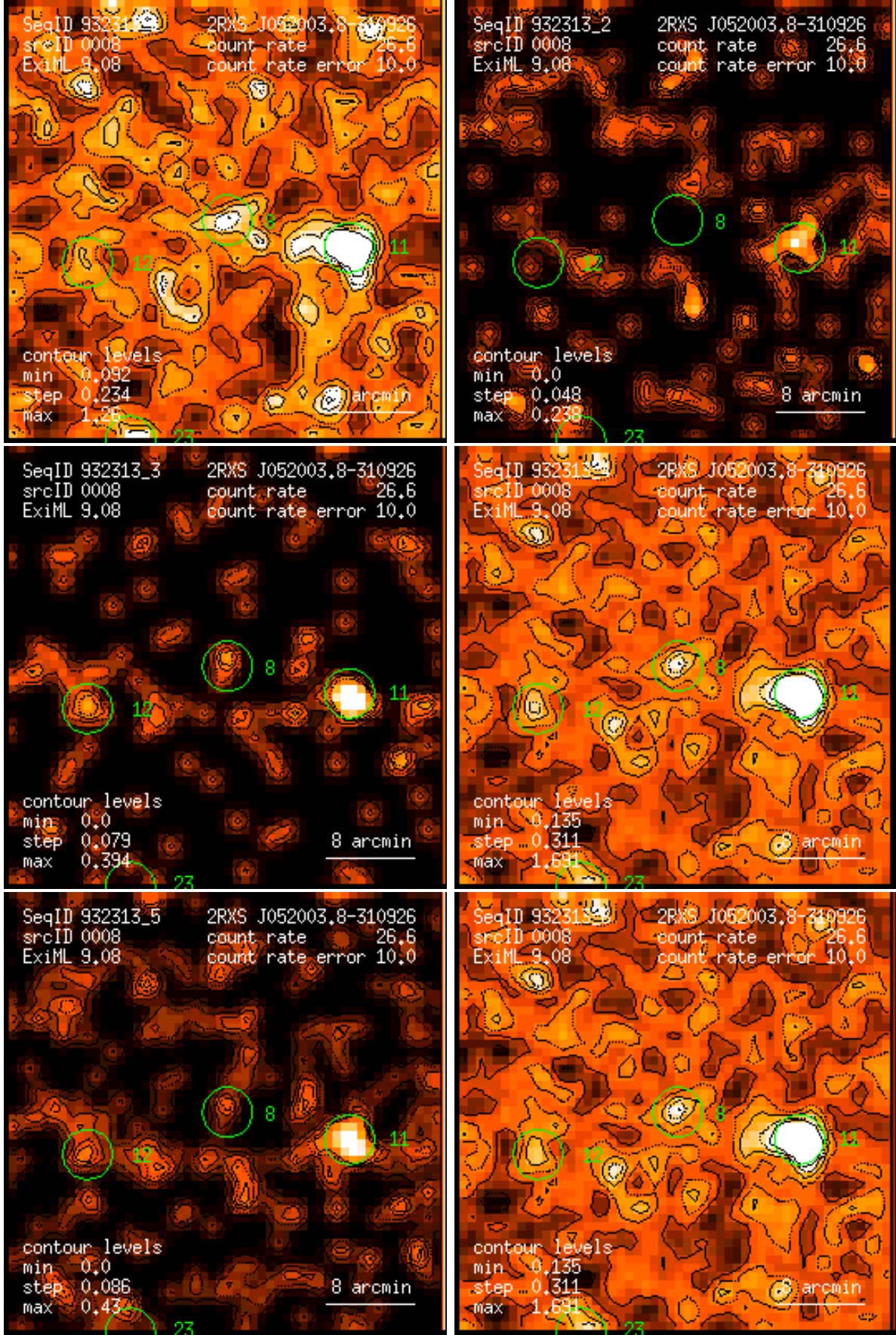
Figure 8: RASS 932313: detection 0008: band rate images, Gaussian filter: (1) PSPC channels 11 – 41, (2) 52 – 90, (3) 91 – 201, (4) 11 – 235, (5) 52 – 201, (6) 11 – 201. Broad band rates in counts/ks. Band rate contour levels in counts/ks/arcmin 2 .
