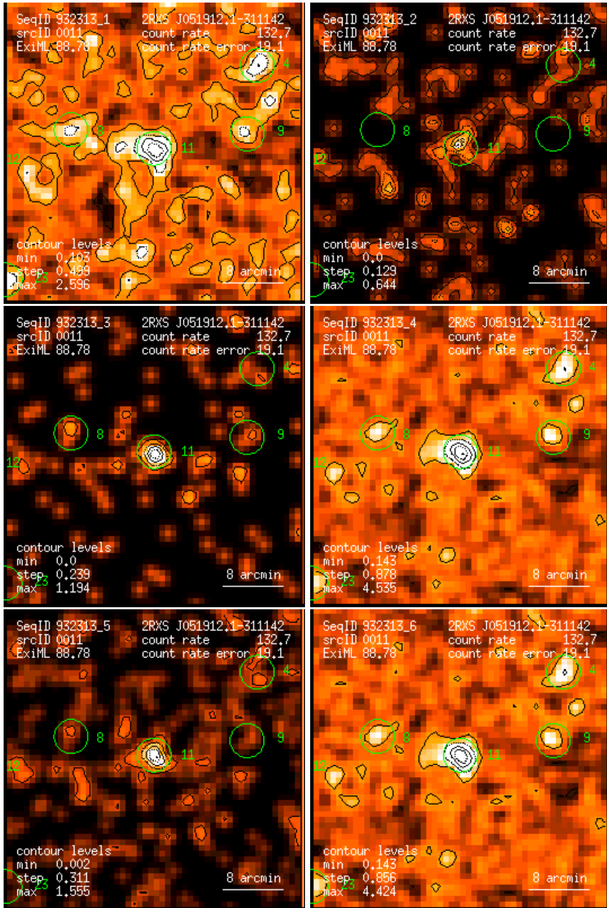
Figure 11: RASS 932313: detection 0011: band rate images, Gaussian filter: (1) PSPC channels 11 – 41, (2) 52 – 90, (3) 91 – 201, (4) 11 – 235, (5) 52 – 201, (6) 11 – 201. Broad band rates in counts/ks. Band rate contour levels in counts/ks/arcmin 2 .
