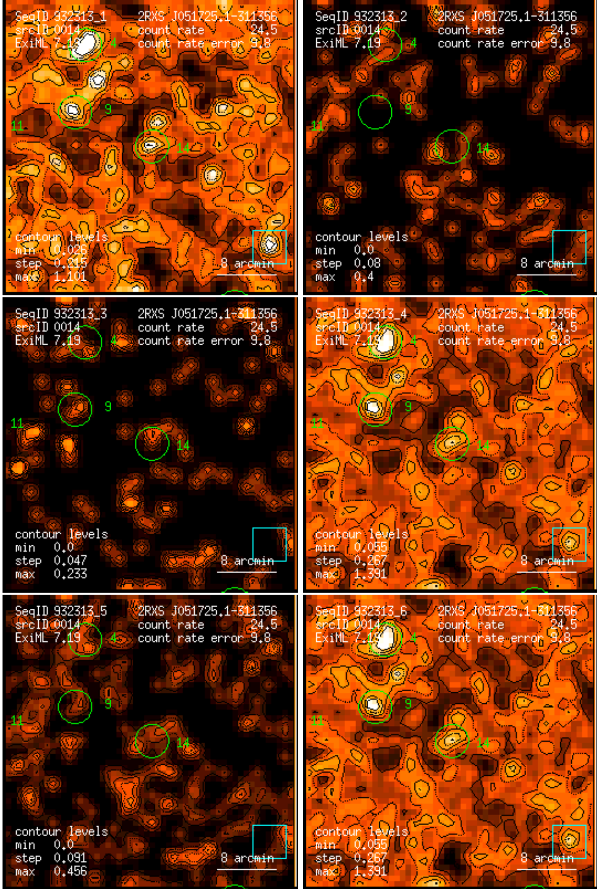
Figure 14: RASS 932313: detection 0014: band rate images, Gaussian filter: (1) PSPC channels 11 – 41, (2) 52 – 90, (3) 91 – 201, (4) 11 – 235, (5) 52 – 201, (6) 11 – 201. Broad band rates in counts/ks. Band rate contour levels in counts/ks/arcmin 2 .
