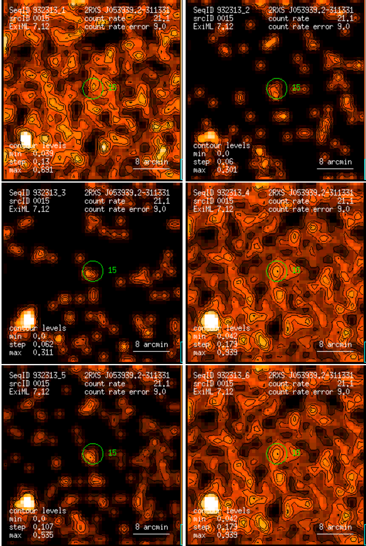
Figure 15: RASS 932313: detection 0015: band rate images, Gaussian filter: (1) PSPC channels 11 – 41, (2) 52 – 90, (3) 91 – 201, (4) 11 – 235, (5) 52 – 201, (6) 11 – 201. Broad band rates in counts/ks. Band rate contour levels in counts/ks/arcmin 2 .
