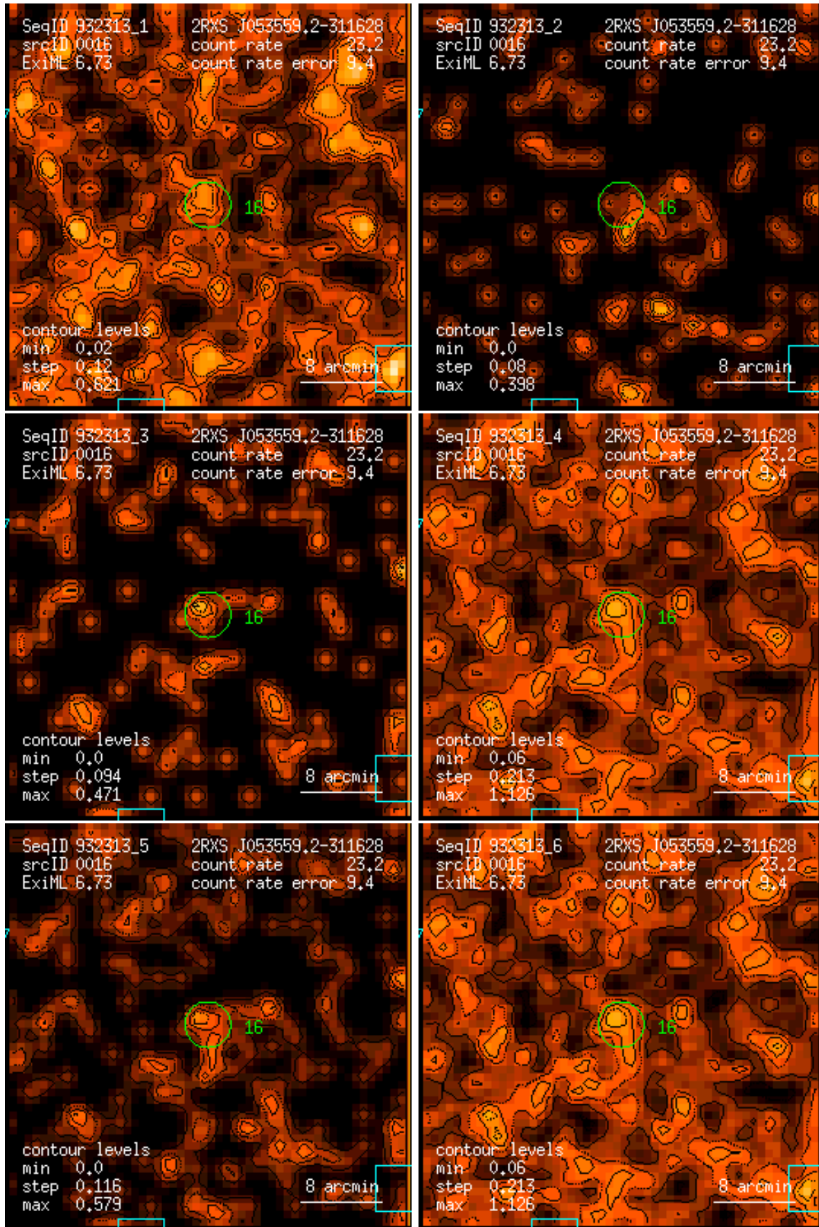
Figure 16: RASS 932313: detection 0016: band rate images, Gaussian filter: (1) PSPC channels 11 – 41, (2) 52 – 90, (3) 91 – 201, (4) 11 – 235, (5) 52 – 201, (6) 11 – 201. Broad band rates in counts/ks. Band rate contour levels in counts/ks/arcmin 2 .
