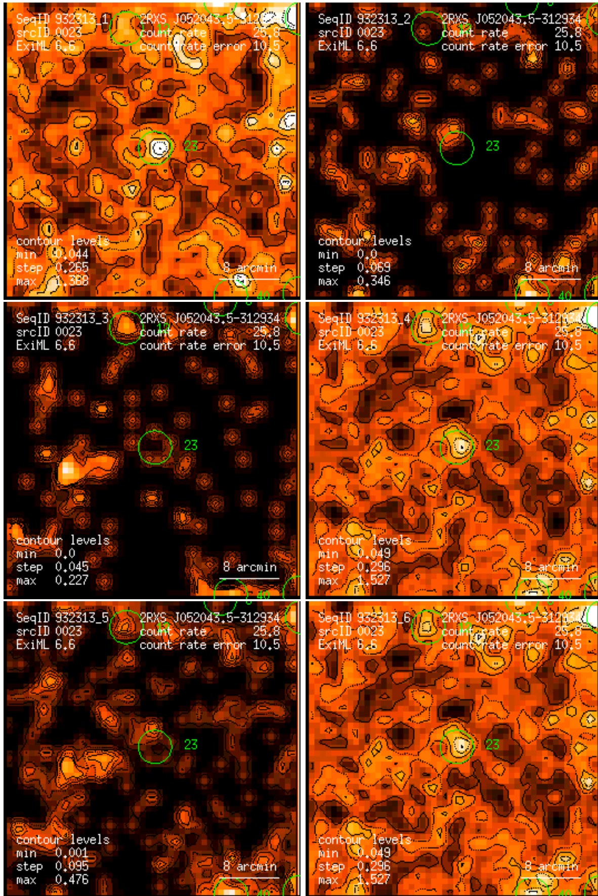
Figure 23: RASS 932313: detection 0023: band rate images, Gaussian filter: (1) PSPC channels 11 – 41, (2) 52 – 90, (3) 91 – 201, (4) 11 – 235, (5) 52 – 201, (6) 11 – 201. Broad band rates in counts/ks. Band rate contour levels in counts/ks/arcmin 2 .
