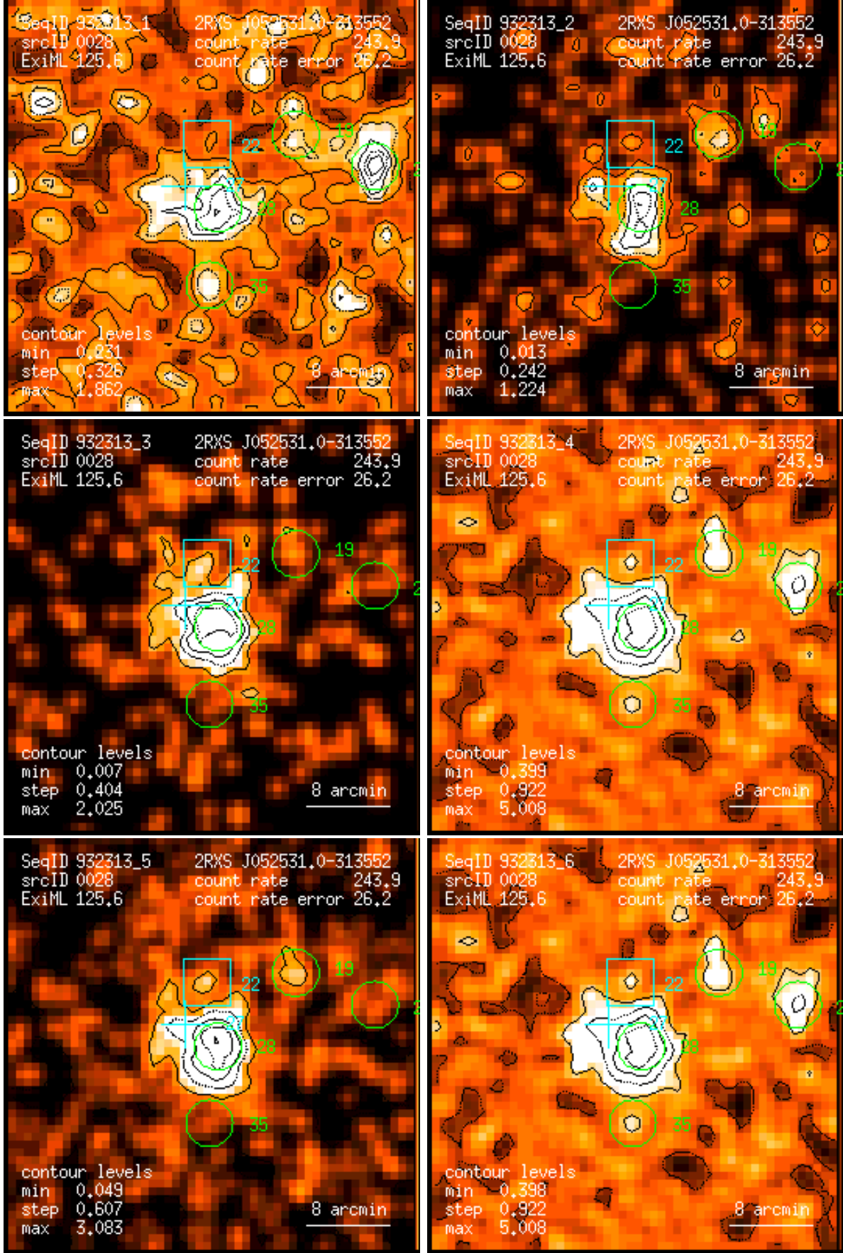
Figure 28: RASS 932313: detection 0028: band rate images, Gaussian filter: (1) PSPC channels 11 – 41, (2) 52 – 90, (3) 91 – 201, (4) 11 – 235, (5) 52 – 201, (6) 11 – 201. Broad band rates in counts/ks. Band rate contour levels in counts/ks/arcmin 2 .
