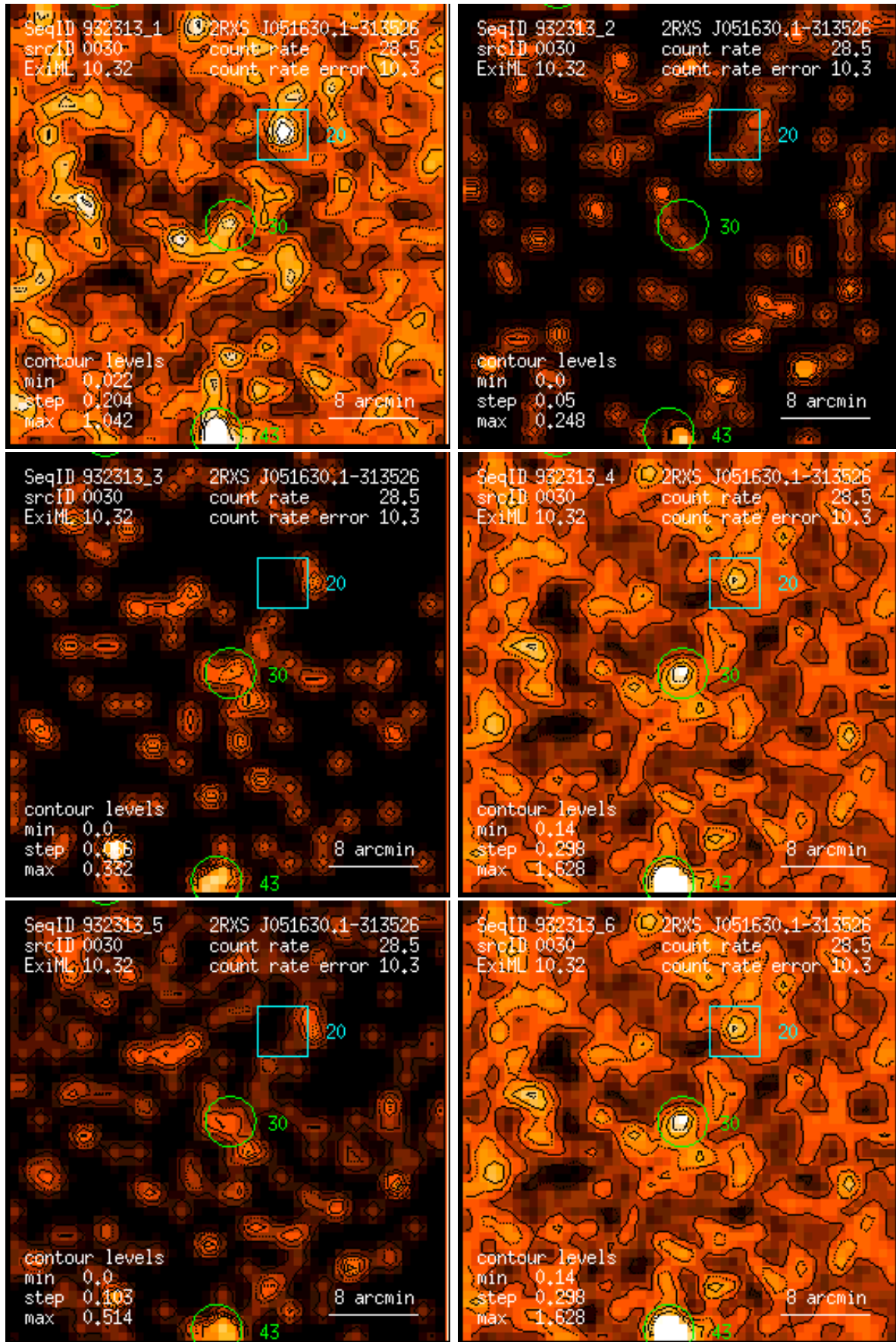
Figure 30: RASS 932313: detection 0030: band rate images, Gaussian filter: (1) PSPC channels 11 – 41, (2) 52 – 90, (3) 91 – 201, (4) 11 – 235, (5) 52 – 201, (6) 11 – 201. Broad band rates in counts/ks. Band rate contour levels in counts/ks/arcmin 2 .
