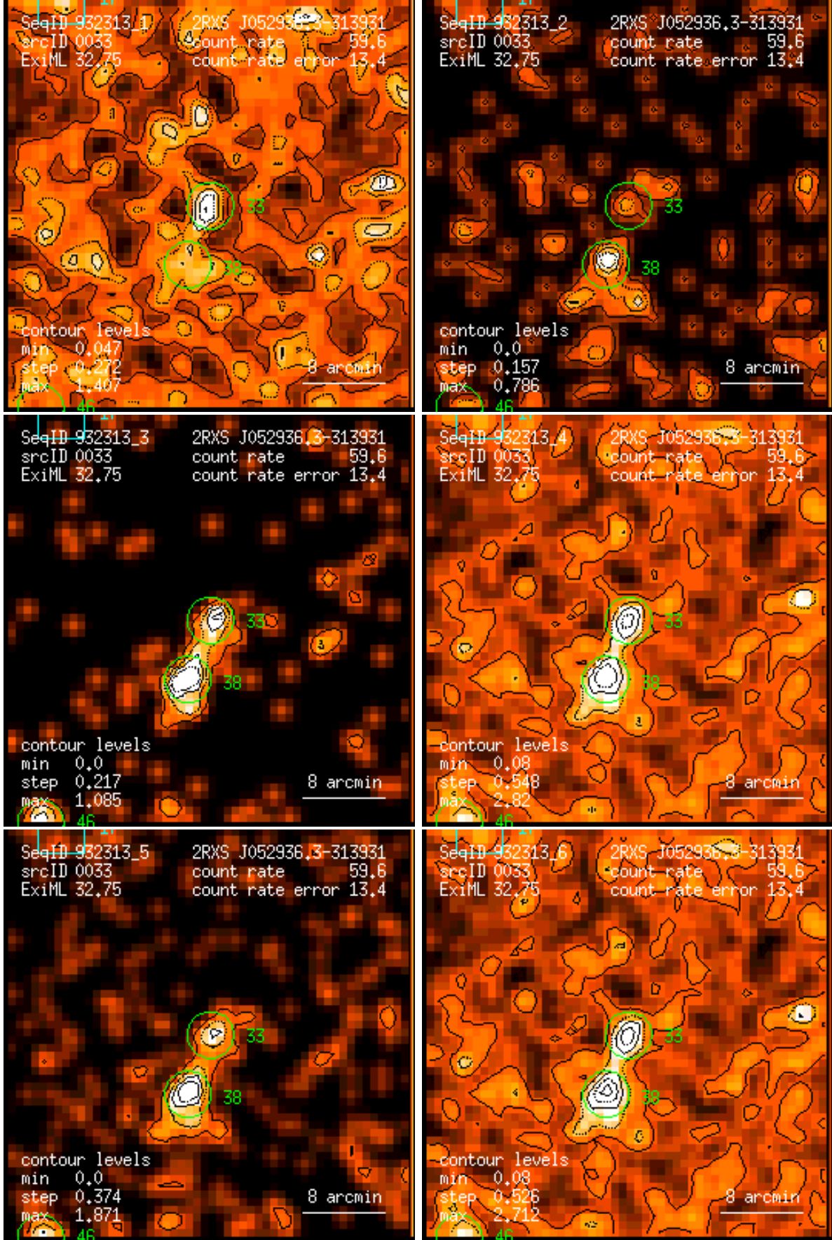
Figure 33: RASS 932313: detection 0033: band rate images, Gaussian filter: (1) PSPC channels 11 – 41, (2) 52 – 90, (3) 91 – 201, (4) 11 – 235, (5) 52 – 201, (6) 11 – 201. Broad band rates in counts/ks. Band rate contour levels in counts/ks/arcmin 2 .
