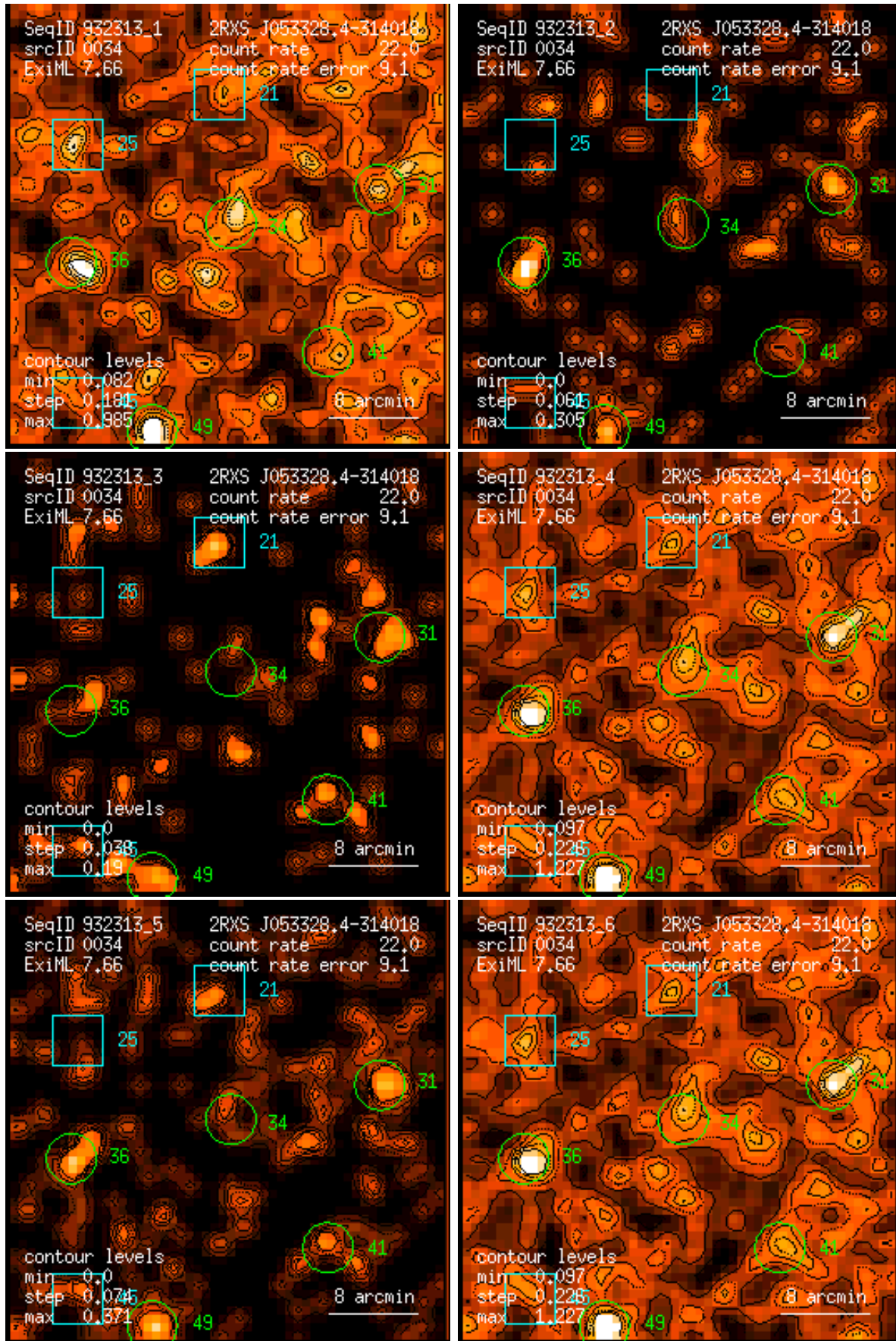
Figure 34: RASS 932313: detection 0034: band rate images, Gaussian filter: (1) PSPC channels 11 – 41, (2) 52 – 90, (3) 91 – 201, (4) 11 – 235, (5) 52 – 201, (6) 11 – 201. Broad band rates in counts/ks. Band rate contour levels in counts/ks/arcmin 2 .
