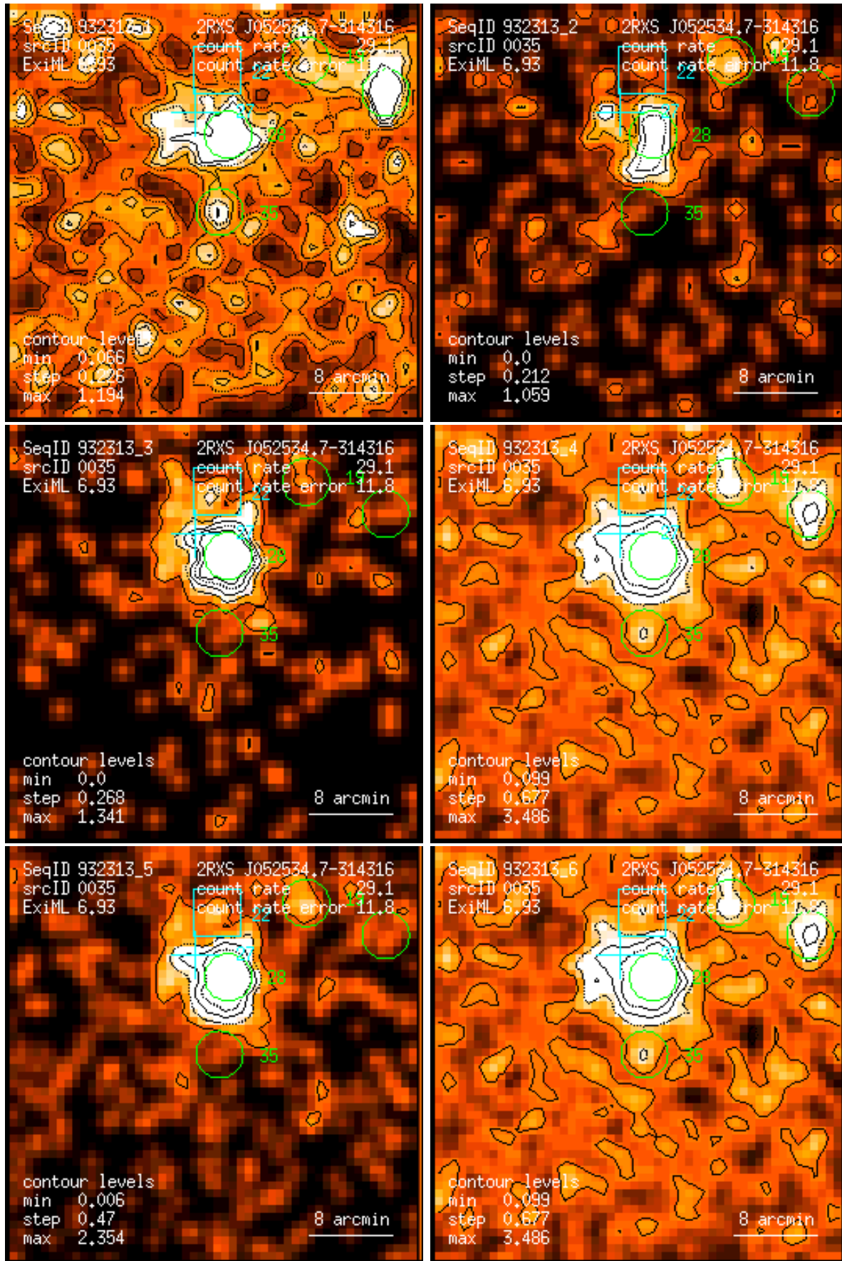
Figure 35: RASS 932313: detection 0035: band rate images, Gaussian filter: (1) PSPC channels 11 – 41, (2) 52 – 90, (3) 91 – 201, (4) 11 – 235, (5) 52 – 201, (6) 11 – 201. Broad band rates in counts/ks. Band rate contour levels in counts/ks/arcmin 2 .
