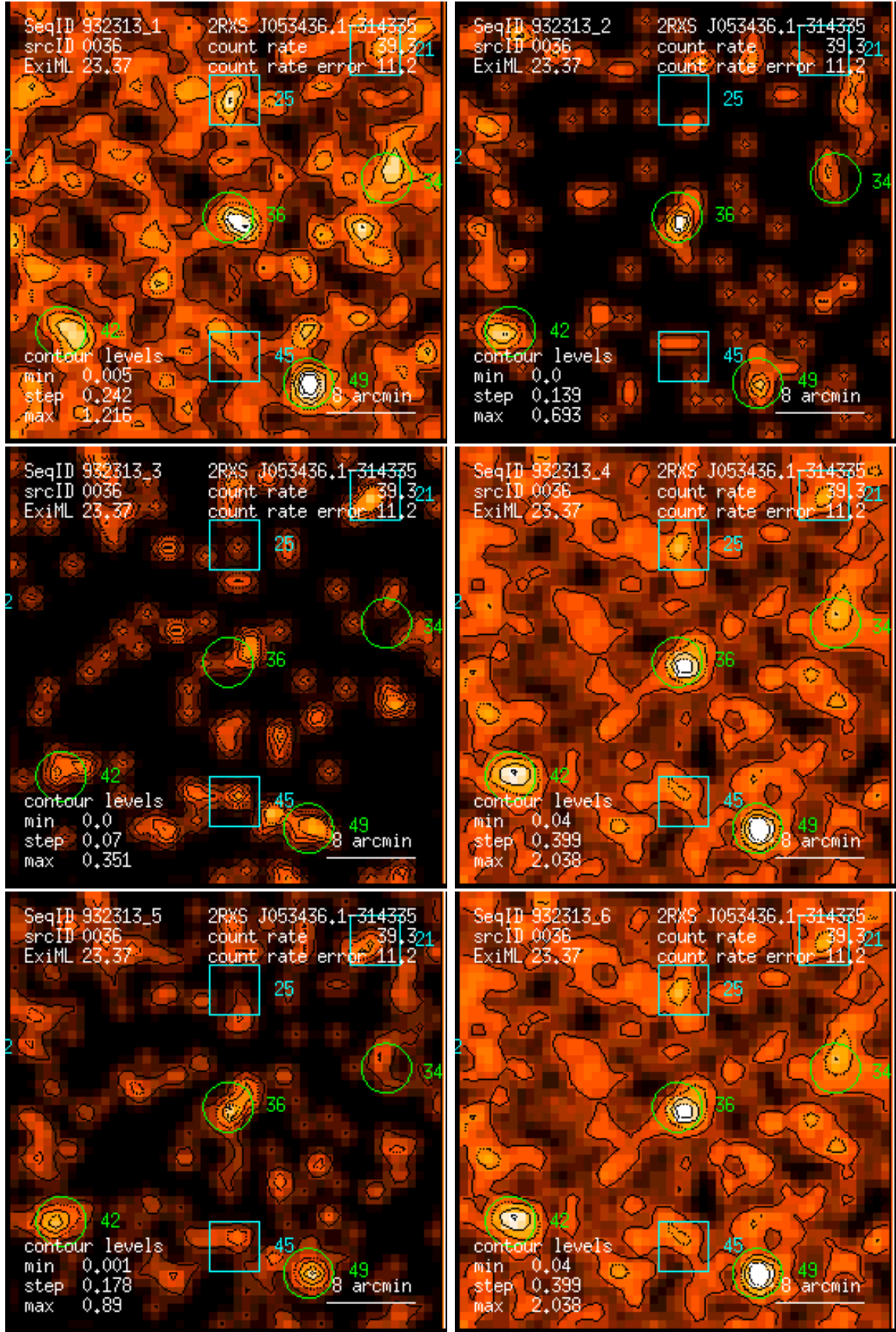
Figure 36: RASS 932313: detection 0036: band rate images, Gaussian filter: (1) PSPC channels 11 – 41, (2) 52 – 90, (3) 91 – 201, (4) 11 – 235, (5) 52 – 201, (6) 11 – 201. Broad band rates in counts/ks. Band rate contour levels in counts/ks/arcmin 2 .
