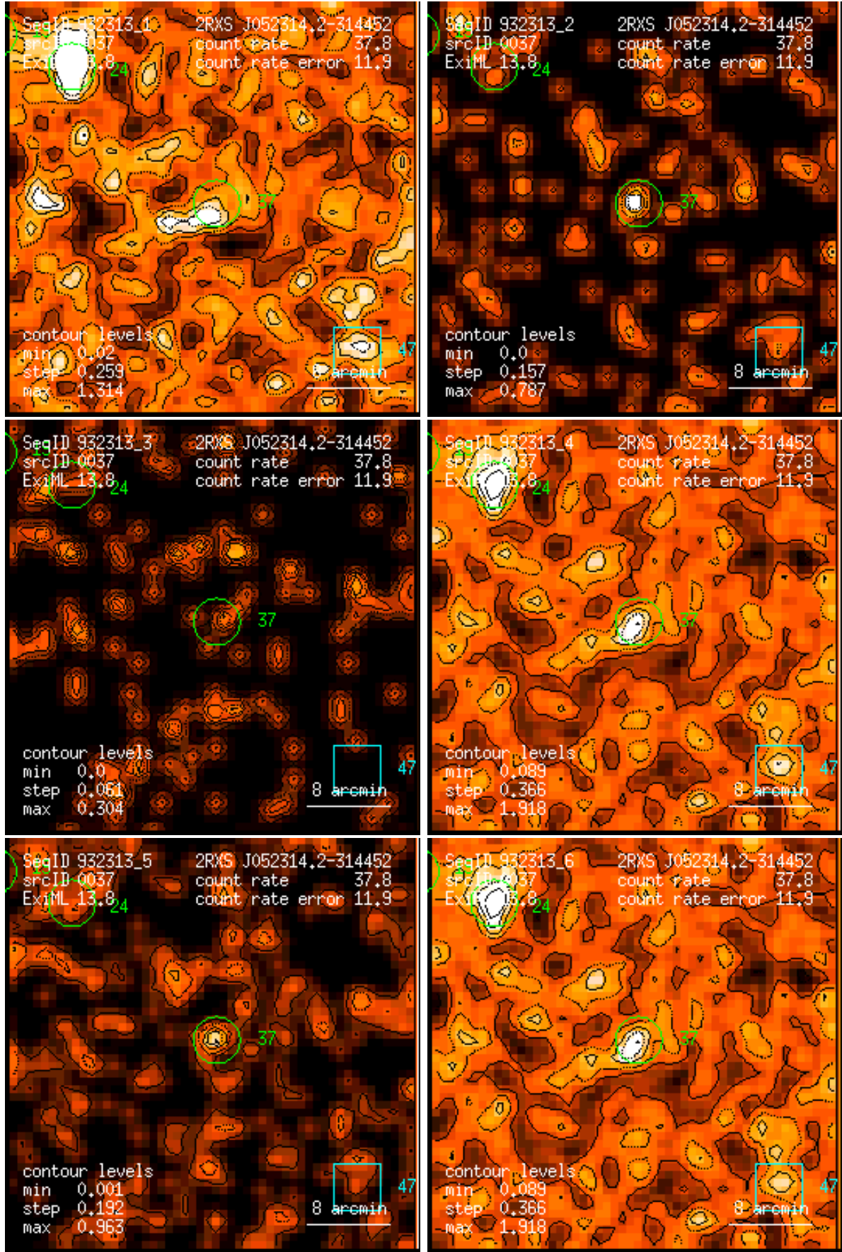
Figure 37: RASS 932313: detection 0037: band rate images, Gaussian filter: (1) PSPC channels 11 – 41, (2) 52 – 90, (3) 91 – 201, (4) 11 – 235, (5) 52 – 201, (6) 11 – 201. Broad band rates in counts/ks. Band rate contour levels in counts/ks/arcmin 2 .
