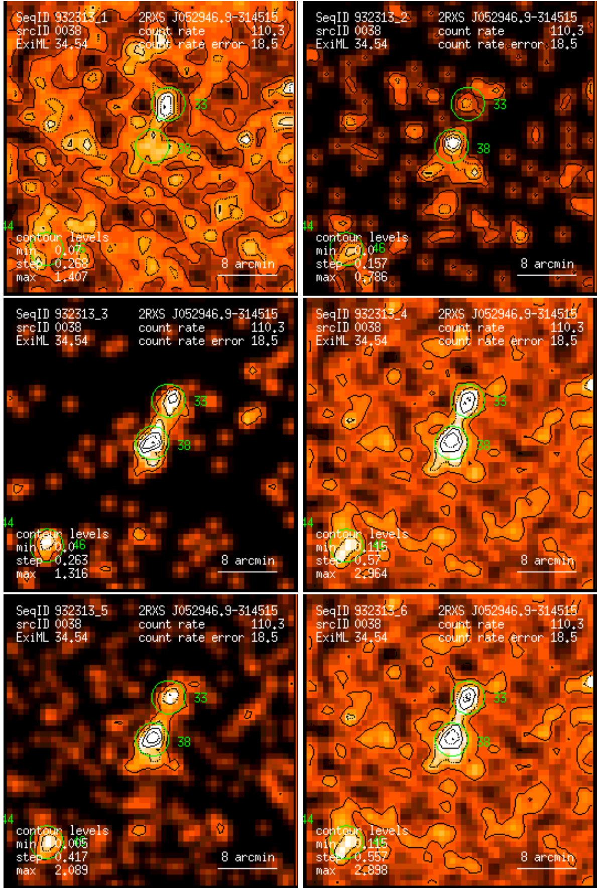
Figure 38: RASS 932313: detection 0038: band rate images, Gaussian filter: (1) PSPC channels 11 – 41, (2) 52 – 90, (3) 91 – 201, (4) 11 – 235, (5) 52 – 201, (6) 11 – 201. Broad band rates in counts/ks. Band rate contour levels in counts/ks/arcmin 2 .
