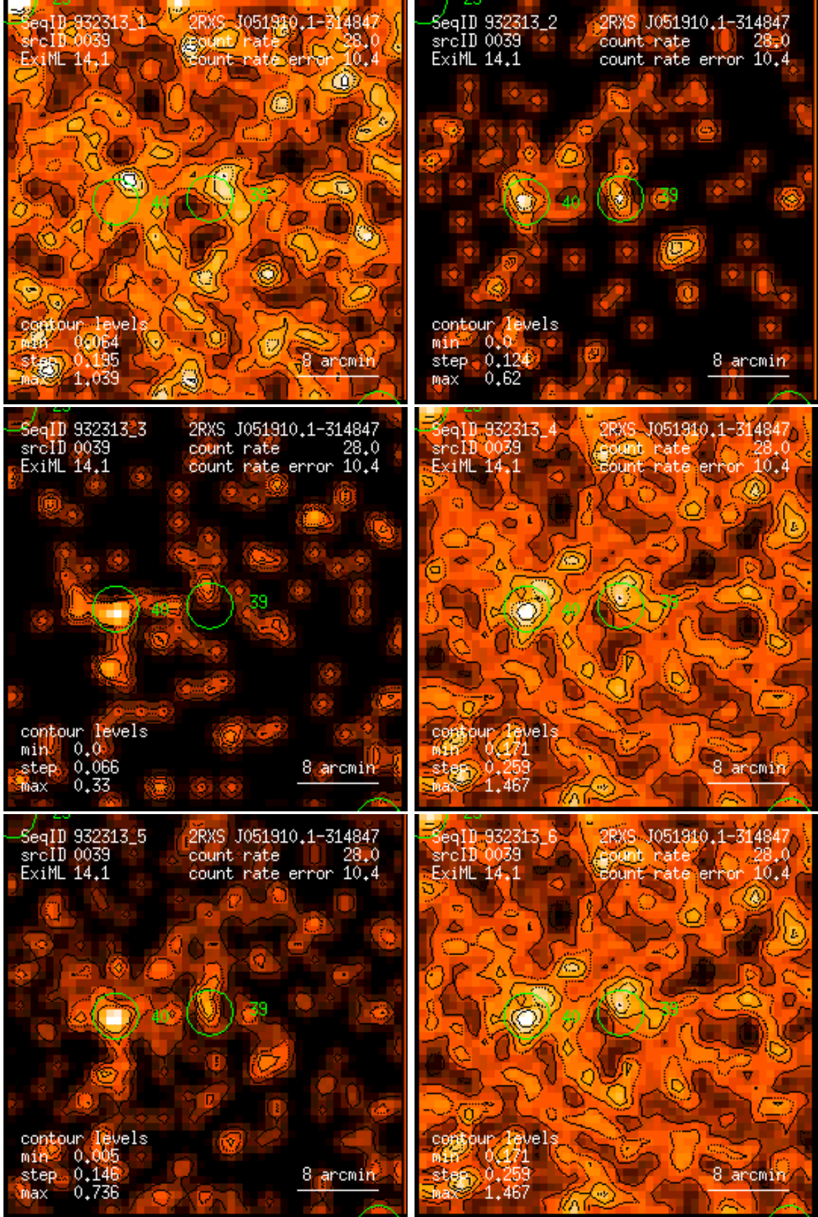
Figure 39: RASS 932313: detection 0039: band rate images, Gaussian filter: (1) PSPC channels 11 – 41, (2) 52 – 90, (3) 91 – 201, (4) 11 – 235, (5) 52 – 201, (6) 11 – 201. Broad band rates in counts/ks. Band rate contour levels in counts/ks/arcmin 2 .
