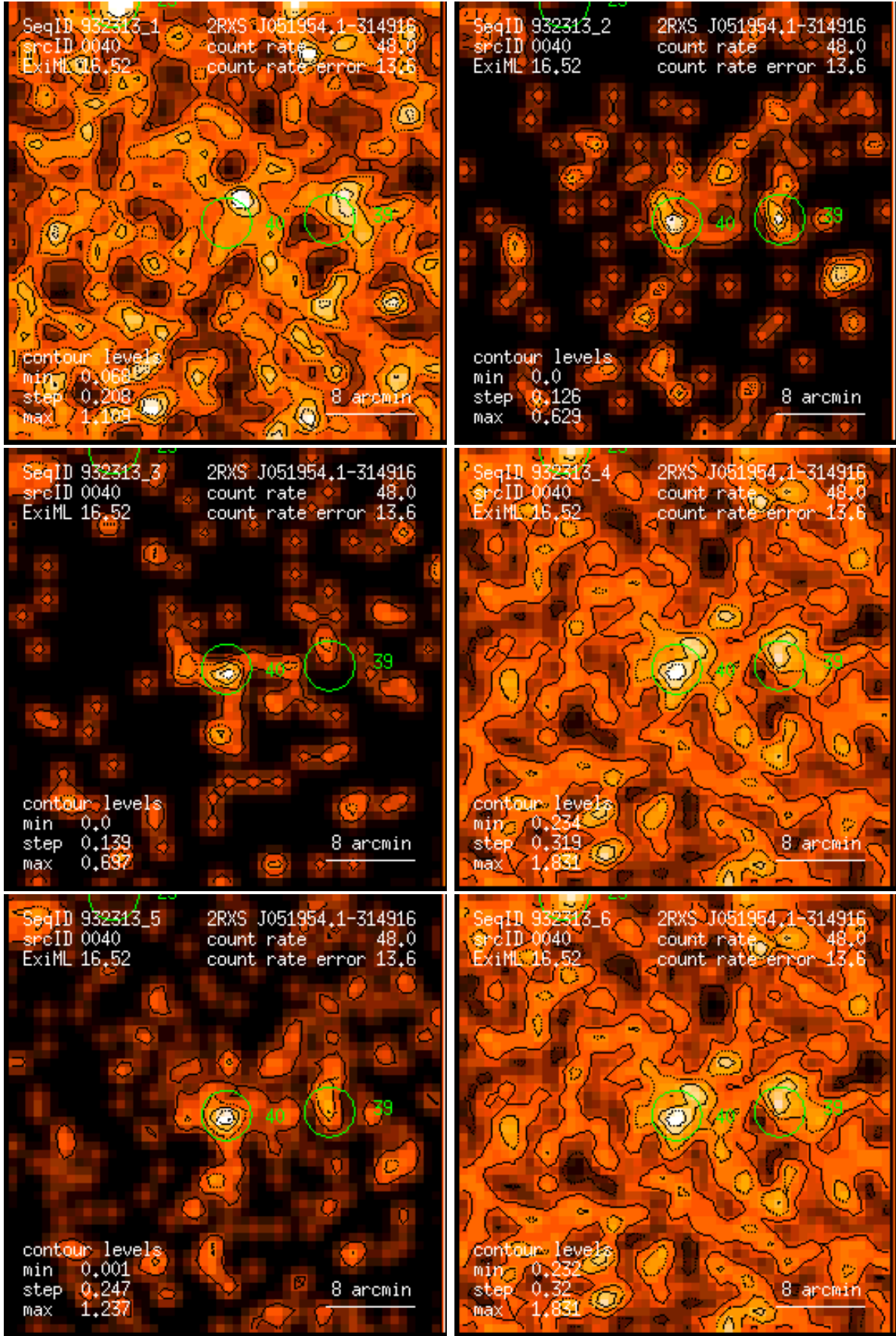
Figure 40: RASS 932313: detection 0040: band rate images, Gaussian filter: (1) PSPC channels 11 – 41, (2) 52 – 90, (3) 91 – 201, (4) 11 – 235, (5) 52 – 201, (6) 11 – 201. Broad band rates in counts/ks. Band rate contour levels in counts/ks/arcmin 2 .
