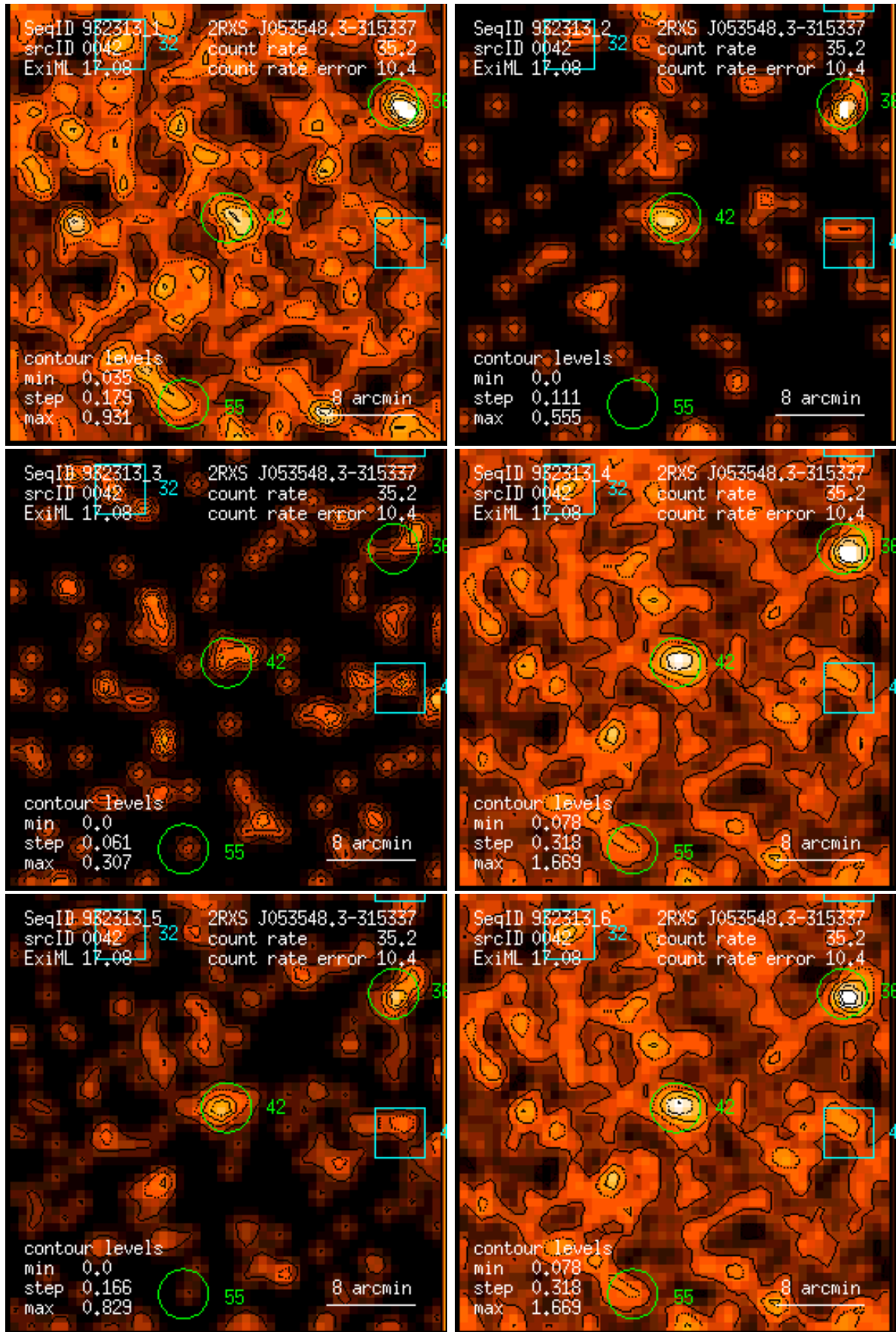
Figure 42: RASS 932313: detection 0042: band rate images, Gaussian filter: (1) PSPC channels 11 – 41, (2) 52 – 90, (3) 91 – 201, (4) 11 – 235, (5) 52 – 201, (6) 11 – 201. Broad band rates in counts/ks. Band rate contour levels in counts/ks/arcmin 2 .
