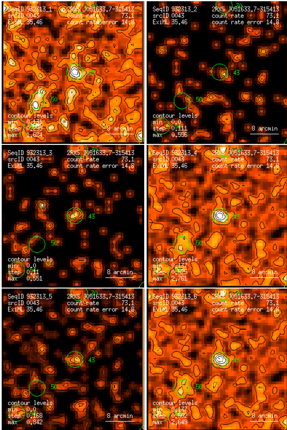
Figure 43: RASS 932313: detection 0043: band rate images, Gaussian filter: (1) PSPC channels 11 – 41, (2) 52 – 90, (3) 91 – 201, (4) 11 – 235, (5) 52 – 201, (6) 11 – 201. Broad band rates in counts/ks. Band rate contour levels in counts/ks/arcmin 2 .
