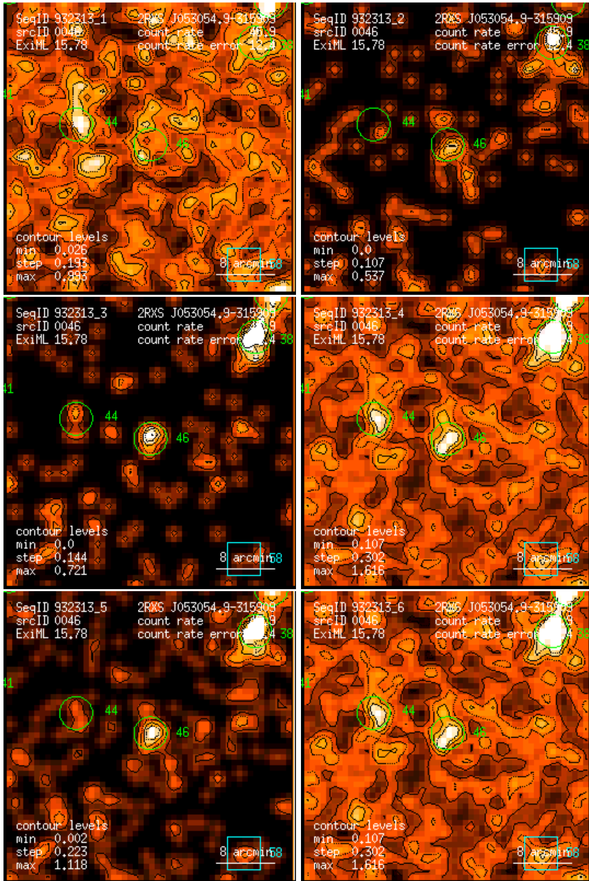
Figure 46: RASS 932313: detection 0046: band rate images, Gaussian filter: (1) PSPC channels 11 – 41, (2) 52 – 90, (3) 91 – 201, (4) 11 – 235, (5) 52 – 201, (6) 11 – 201. Broad band rates in counts/ks. Band rate contour levels in counts/ks/arcmin 2 .
