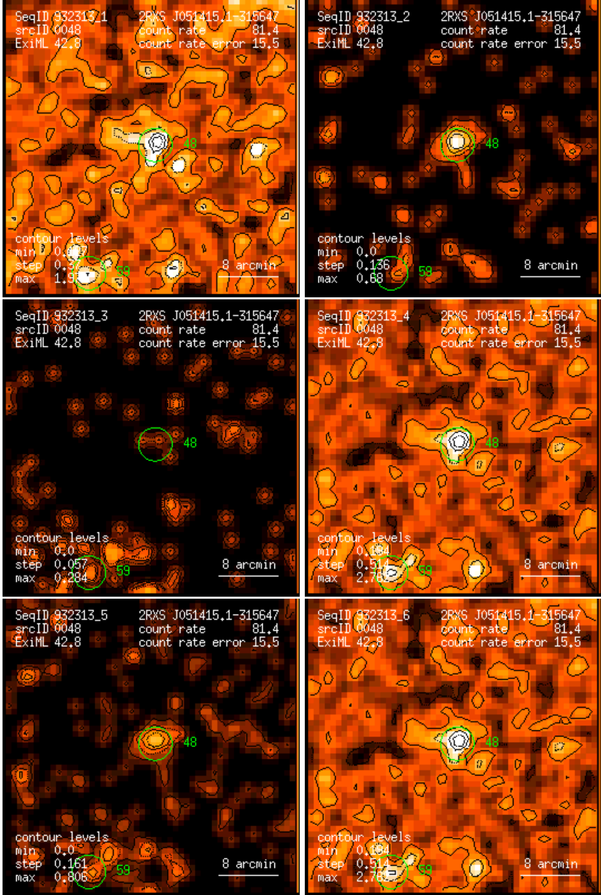
Figure 48: RASS 932313: detection 0048: band rate images, Gaussian filter: (1) PSPC channels 11 – 41, (2) 52 – 90, (3) 91 – 201, (4) 11 – 235, (5) 52 – 201, (6) 11 – 201. Broad band rates in counts/ks. Band rate contour levels in counts/ks/arcmin 2 .
