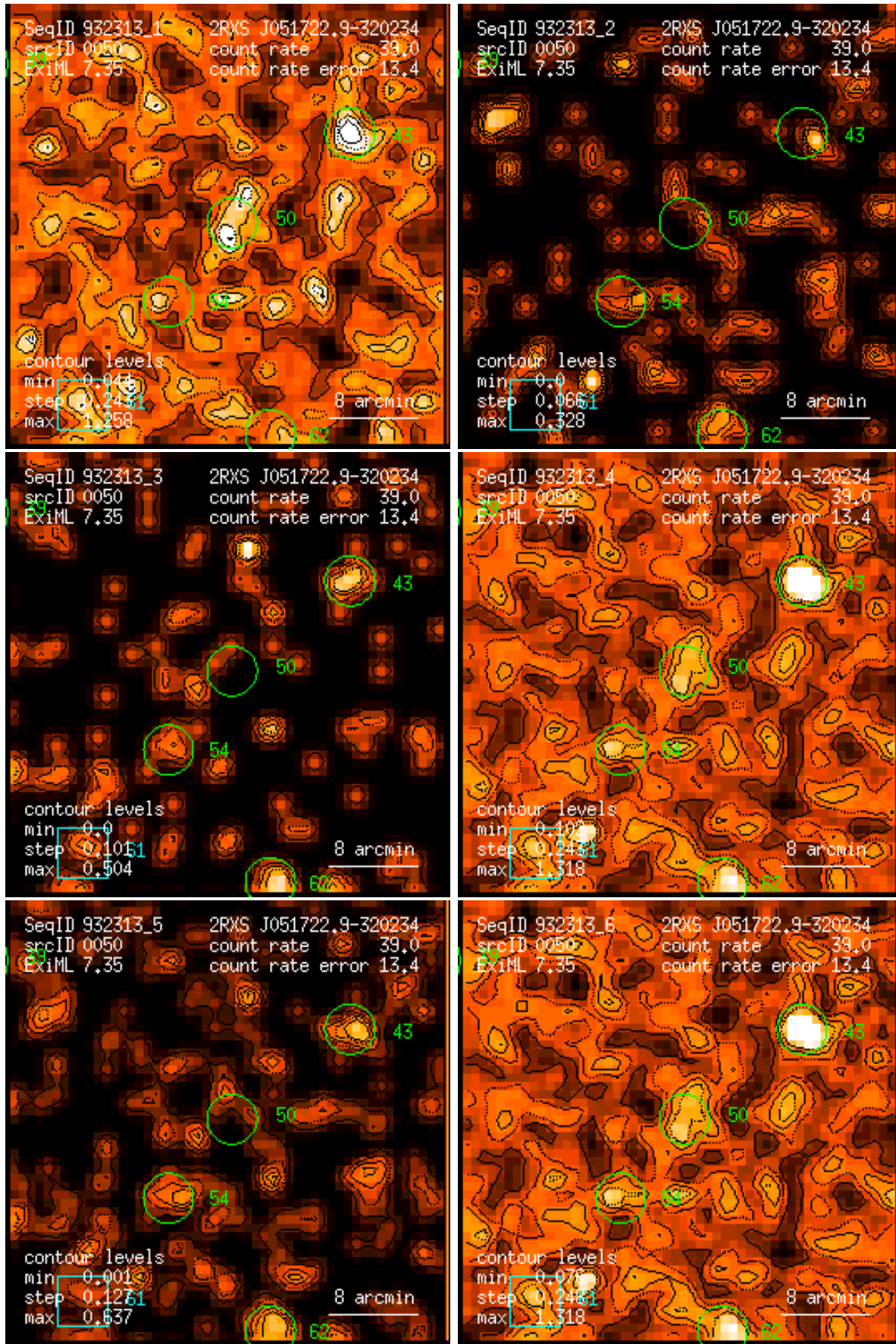
Figure 50: RASS 932313: detection 0050: band rate images, Gaussian filter: (1) PSPC channels 11 – 41, (2) 52 – 90, (3) 91 – 201, (4) 11 – 235, (5) 52 – 201, (6) 11 – 201. Broad band rates in counts/ks. Band rate contour levels in counts/ks/arcmin 2 .
