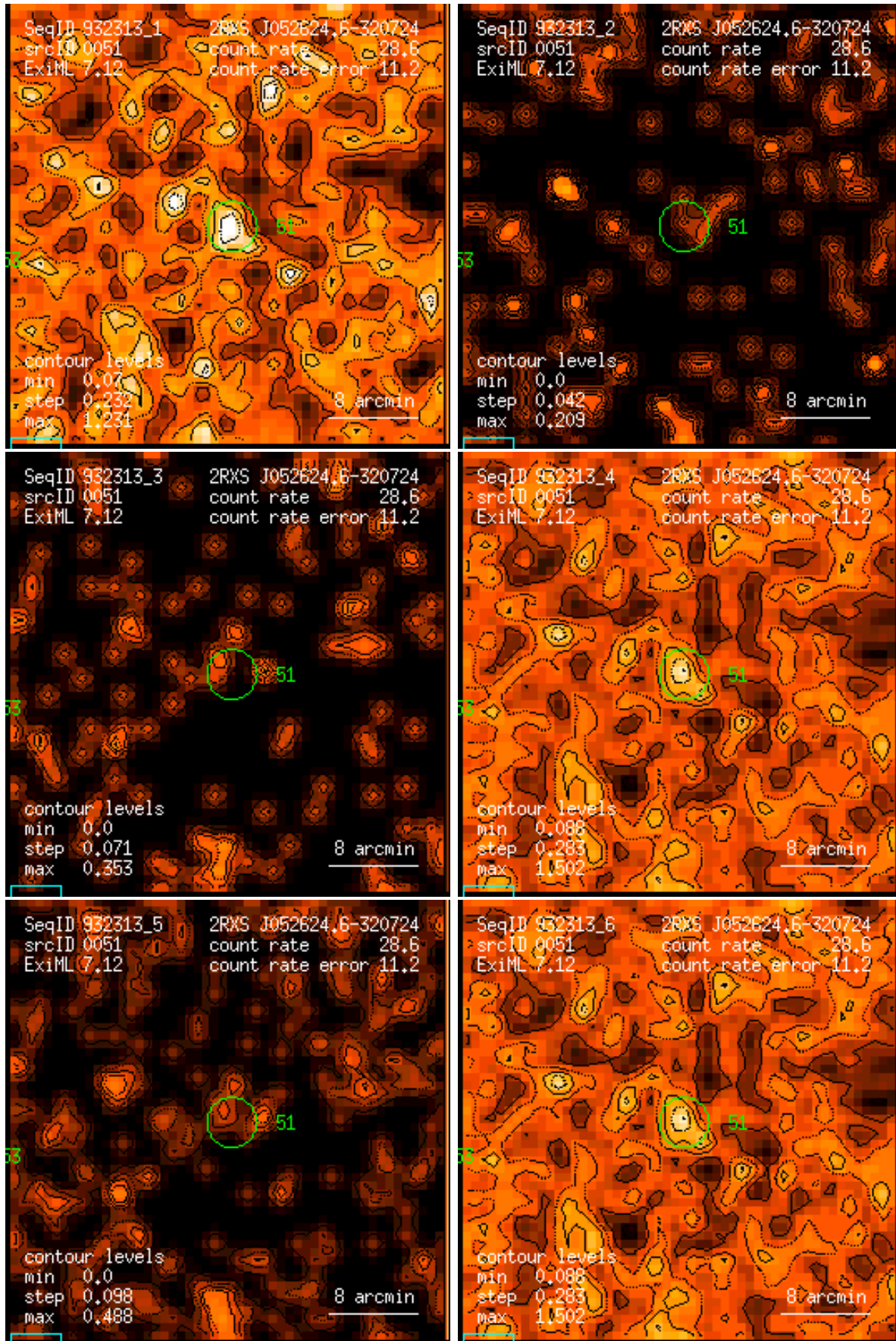
Figure 51: RASS 932313: detection 0051: band rate images, Gaussian filter: (1) PSPC channels 11 – 41, (2) 52 – 90, (3) 91 – 201, (4) 11 – 235, (5) 52 – 201, (6) 11 – 201. Broad band rates in counts/ks. Band rate contour levels in counts/ks/arcmin 2 .
