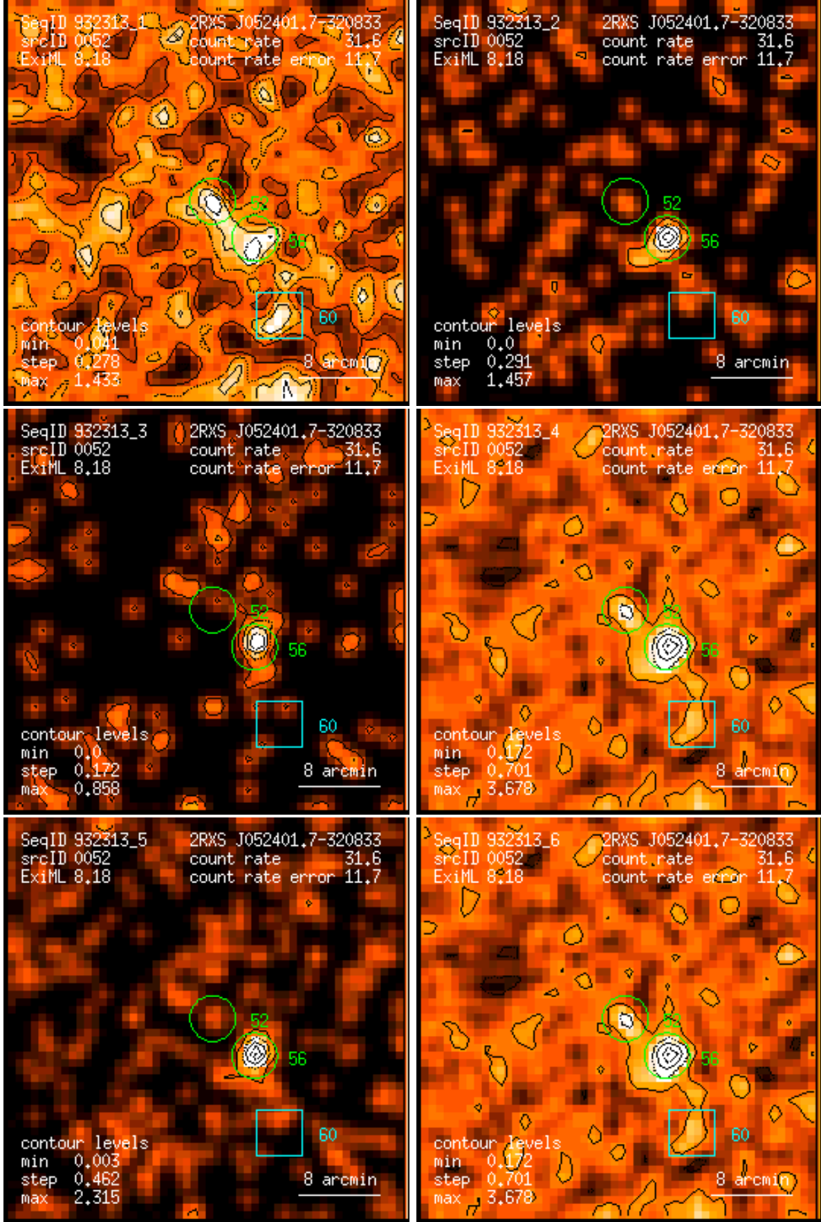
Figure 52: RASS 932313: detection 0052: band rate images, Gaussian filter: (1) PSPC channels 11 – 41, (2) 52 – 90, (3) 91 – 201, (4) 11 – 235, (5) 52 – 201, (6) 11 – 201. Broad band rates in counts/ks. Band rate contour levels in counts/ks/arcmin 2 .
