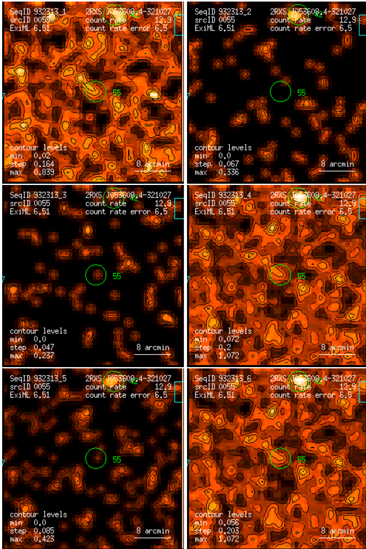
Figure 55: RASS 932313: detection 0055: band rate images, Gaussian filter: (1) PSPC channels 11 – 41, (2) 52 – 90, (3) 91 – 201, (4) 11 – 235, (5) 52 – 201, (6) 11 – 201. Broad band rates in counts/ks. Band rate contour levels in counts/ks/arcmin 2 .
