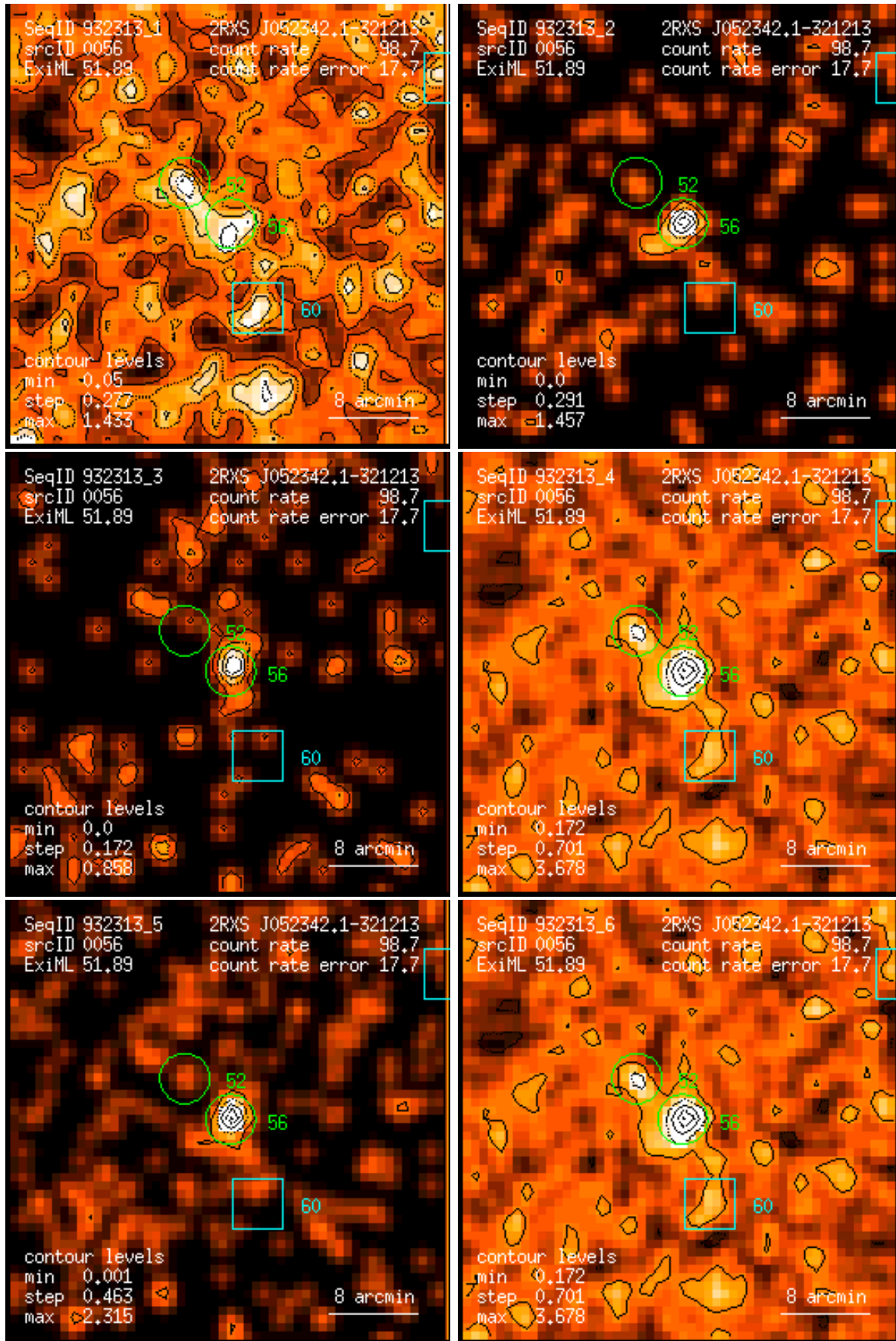
Figure 56: RASS 932313: detection 0056: band rate images, Gaussian filter: (1) PSPC channels 11 – 41, (2) 52 – 90, (3) 91 – 201, (4) 11 – 235, (5) 52 – 201, (6) 11 – 201. Broad band rates in counts/ks. Band rate contour levels in counts/ks/arcmin 2 .
