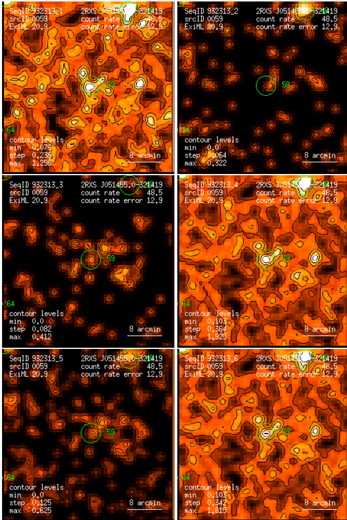
Figure 59: RASS 932313: detection 0059: band rate images, Gaussian filter: (1) PSPC channels 11 – 41, (2) 52 – 90, (3) 91 – 201, (4) 11 – 235, (5) 52 – 201, (6) 11 – 201. Broad band rates in counts/ks. Band rate contour levels in counts/ks/arcmin 2 .
