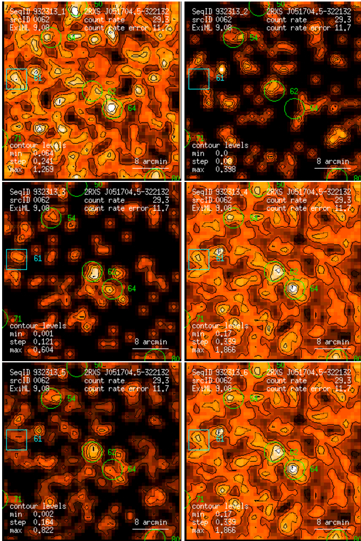
Figure 62: RASS 932313: detection 0062: band rate images, Gaussian filter: (1) PSPC channels 11 – 41, (2) 52 – 90, (3) 91 – 201, (4) 11 – 235, (5) 52 – 201, (6) 11 – 201. Broad band rates in counts/ks. Band rate contour levels in counts/ks/arcmin 2 .
