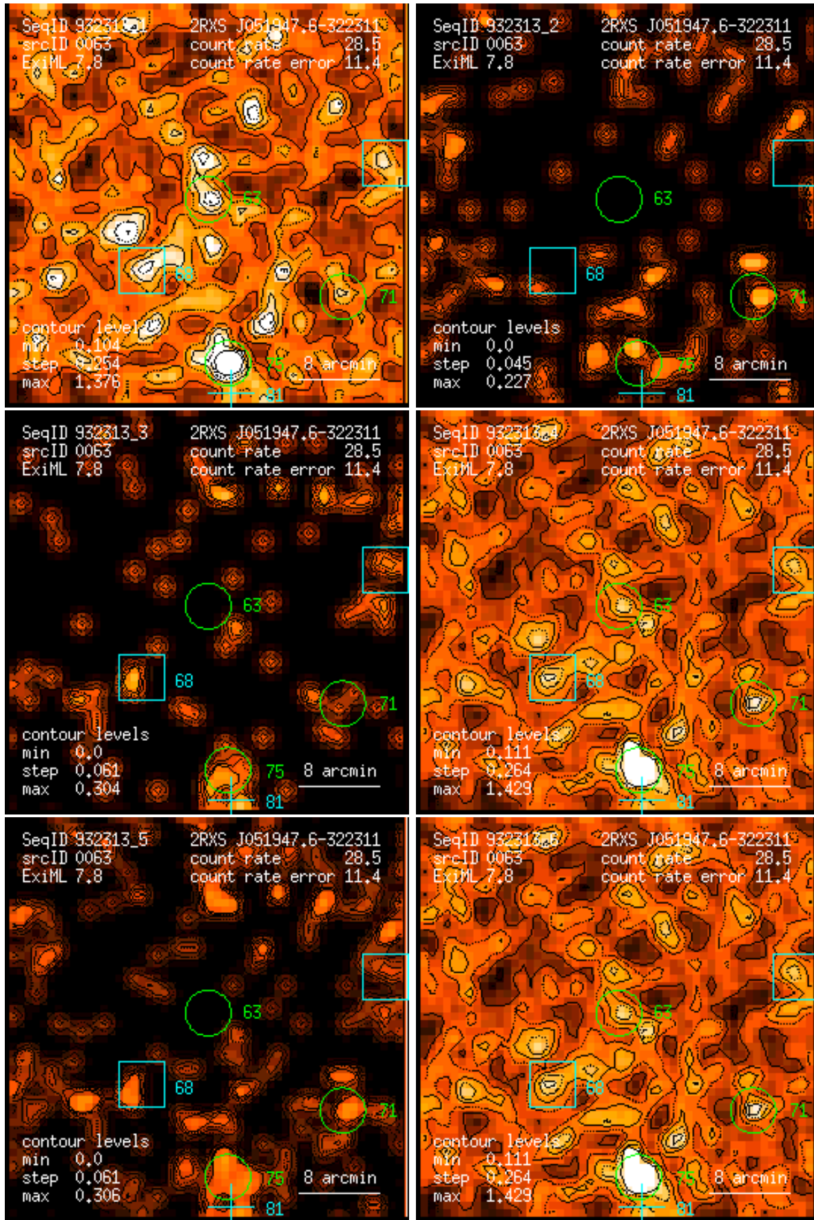
Figure 63: RASS 932313: detection 0063: band rate images, Gaussian filter: (1) PSPC channels 11 – 41, (2) 52 – 90, (3) 91 – 201, (4) 11 – 235, (5) 52 – 201, (6) 11 – 201. Broad band rates in counts/ks. Band rate contour levels in counts/ks/arcmin 2 .
