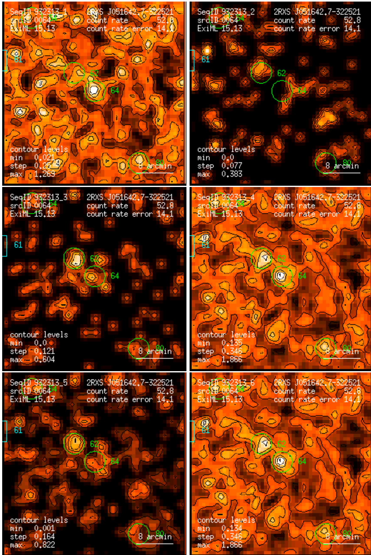
Figure 64: RASS 932313: detection 0064: band rate images, Gaussian filter: (1) PSPC channels 11 – 41, (2) 52 – 90, (3) 91 – 201, (4) 11 – 235, (5) 52 – 201, (6) 11 – 201. Broad band rates in counts/ks. Band rate contour levels in counts/ks/arcmin 2 .
