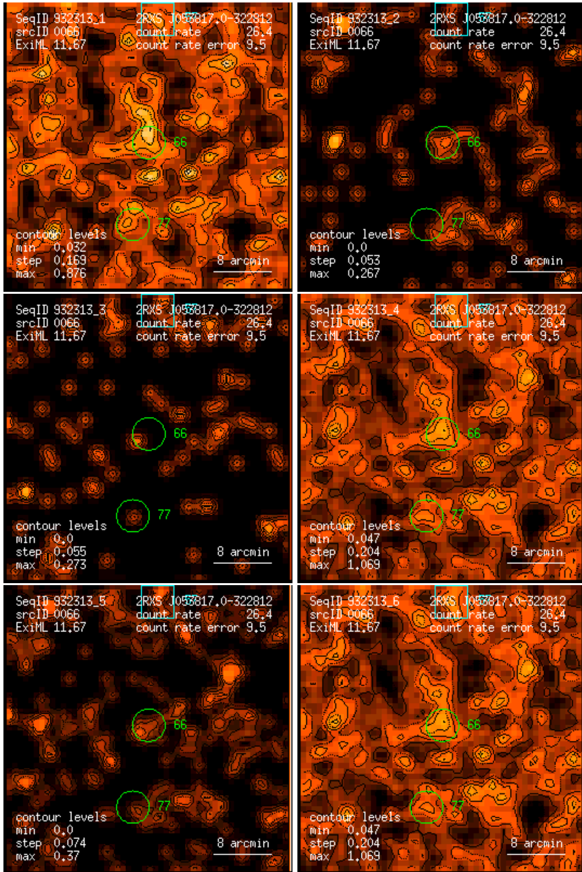
Figure 66: RASS 932313: detection 0066: band rate images, Gaussian filter: (1) PSPC channels 11 – 41, (2) 52 – 90, (3) 91 – 201, (4) 11 – 235, (5) 52 – 201, (6) 11 – 201. Broad band rates in counts/ks. Band rate contour levels in counts/ks/arcmin 2 .
