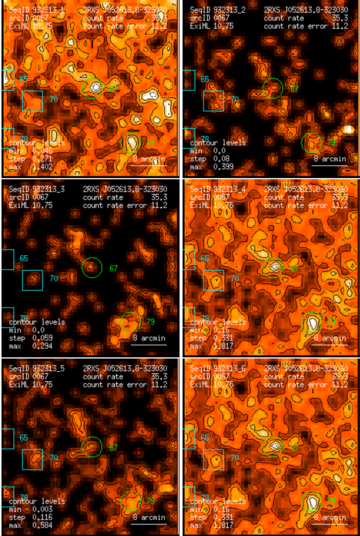
Figure 67: RASS 932313: detection 0067: band rate images, Gaussian filter: (1) PSPC channels 11 – 41, (2) 52 – 90, (3) 91 – 201, (4) 11 – 235, (5) 52 – 201, (6) 11 – 201. Broad band rates in counts/ks. Band rate contour levels in counts/ks/arcmin 2 .
