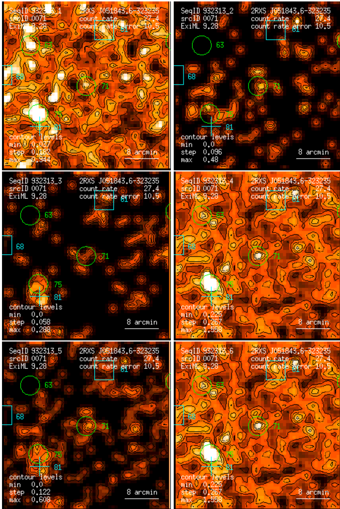
Figure 71: RASS 932313: detection 0071: band rate images, Gaussian filter: (1) PSPC channels 11 – 41, (2) 52 – 90, (3) 91 – 201, (4) 11 – 235, (5) 52 – 201, (6) 11 – 201. Broad band rates in counts/ks. Band rate contour levels in counts/ks/arcmin 2 .
