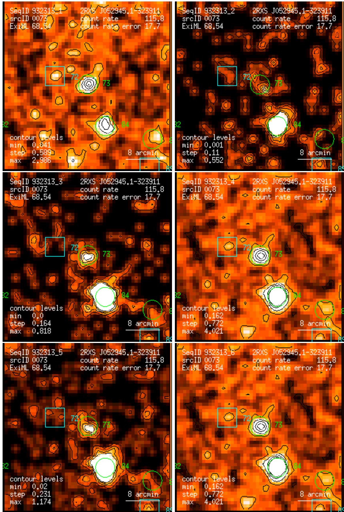
Figure 73: RASS 932313: detection 0073: band rate images, Gaussian filter: (1) PSPC channels 11 – 41, (2) 52 – 90, (3) 91 – 201, (4) 11 – 235, (5) 52 – 201, (6) 11 – 201. Broad band rates in counts/ks. Band rate contour levels in counts/ks/arcmin 2 .
