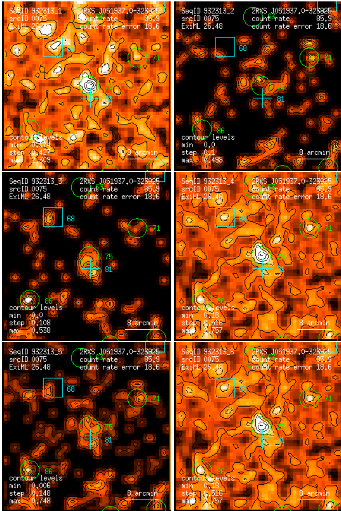
Figure 75: RASS 932313: detection 0075: band rate images, Gaussian filter: (1) PSPC channels 11 – 41, (2) 52 – 90, (3) 91 – 201, (4) 11 – 235, (5) 52 – 201, (6) 11 – 201. Broad band rates in counts/ks. Band rate contour levels in counts/ks/arcmin 2 .
