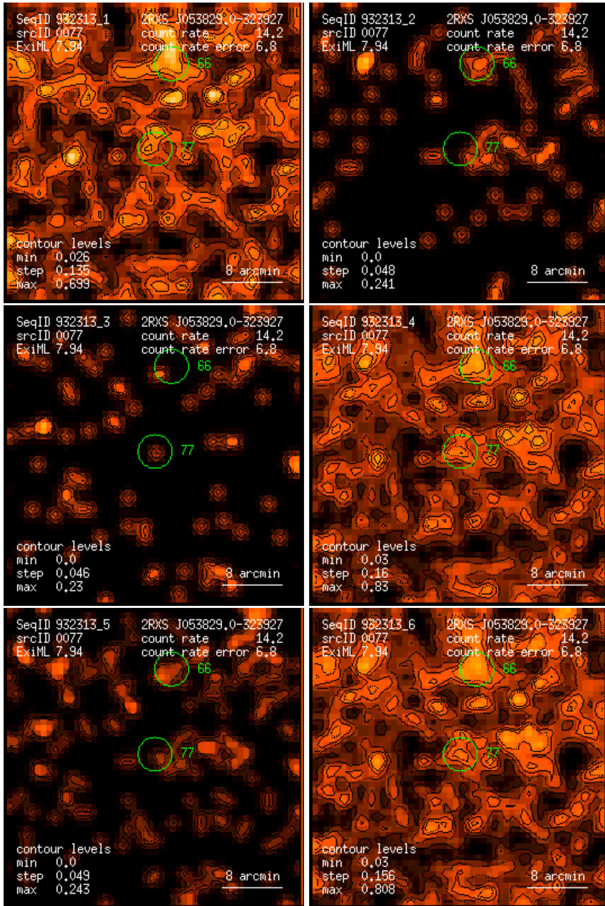
Figure 77: RASS 932313: detection 0077: band rate images, Gaussian filter: (1) PSPC channels 11 – 41, (2) 52 – 90, (3) 91 – 201, (4) 11 – 235, (5) 52 – 201, (6) 11 – 201. Broad band rates in counts/ks. Band rate contour levels in counts/ks/arcmin 2 .
