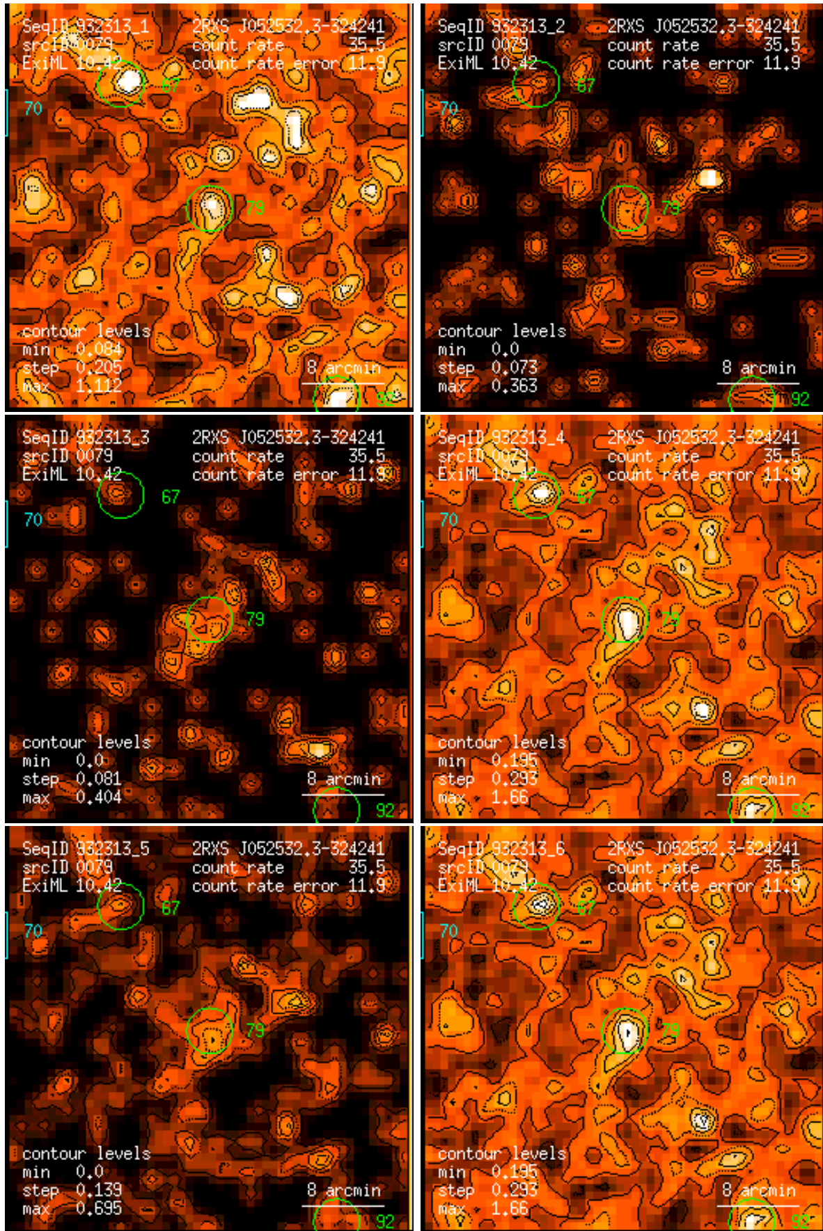
Figure 79: RASS 932313: detection 0079: band rate images, Gaussian filter: (1) PSPC channels 11 – 41, (2) 52 – 90, (3) 91 – 201, (4) 11 – 235, (5) 52 – 201, (6) 11 – 201. Broad band rates in counts/ks. Band rate contour levels in counts/ks/arcmin 2 .
