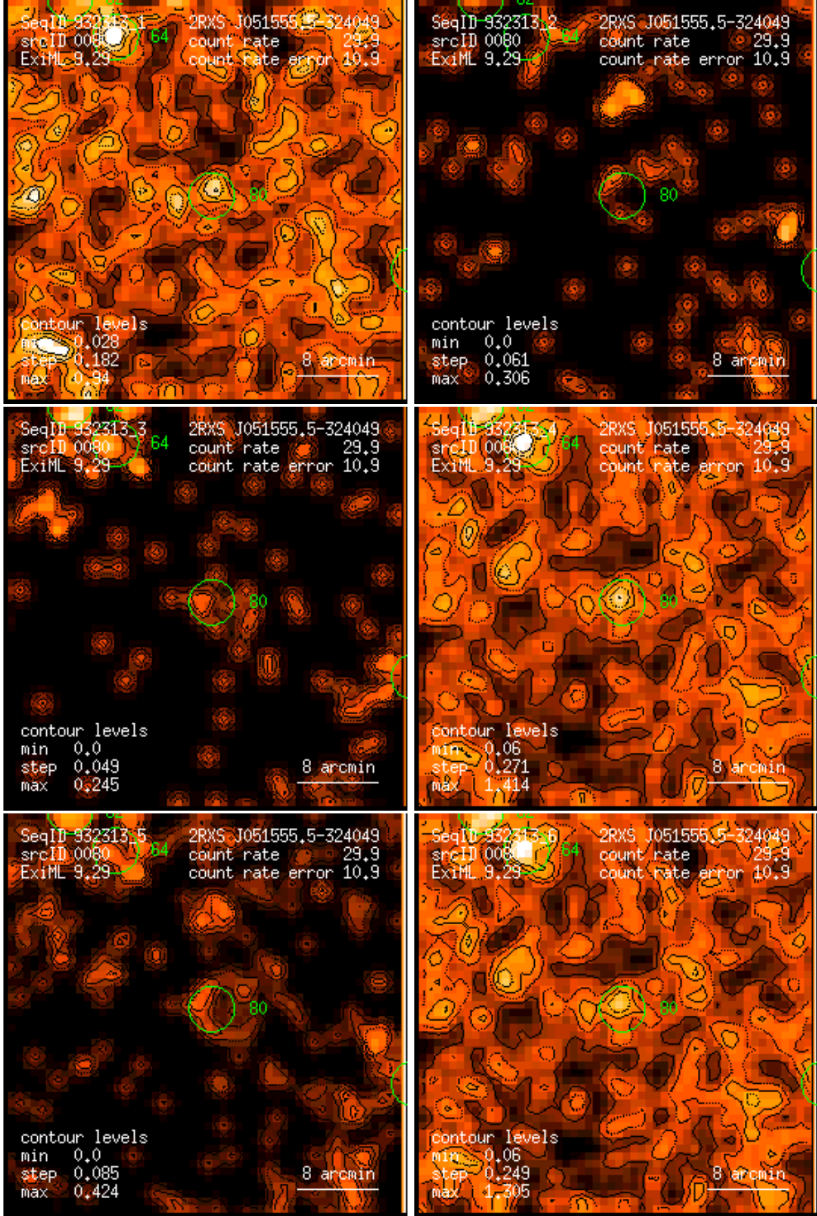
Figure 80: RASS 932313: detection 0080: band rate images, Gaussian filter: (1) PSPC channels 11 – 41, (2) 52 – 90, (3) 91 – 201, (4) 11 – 235, (5) 52 – 201, (6) 11 – 201. Broad band rates in counts/ks. Band rate contour levels in counts/ks/arcmin 2 .
