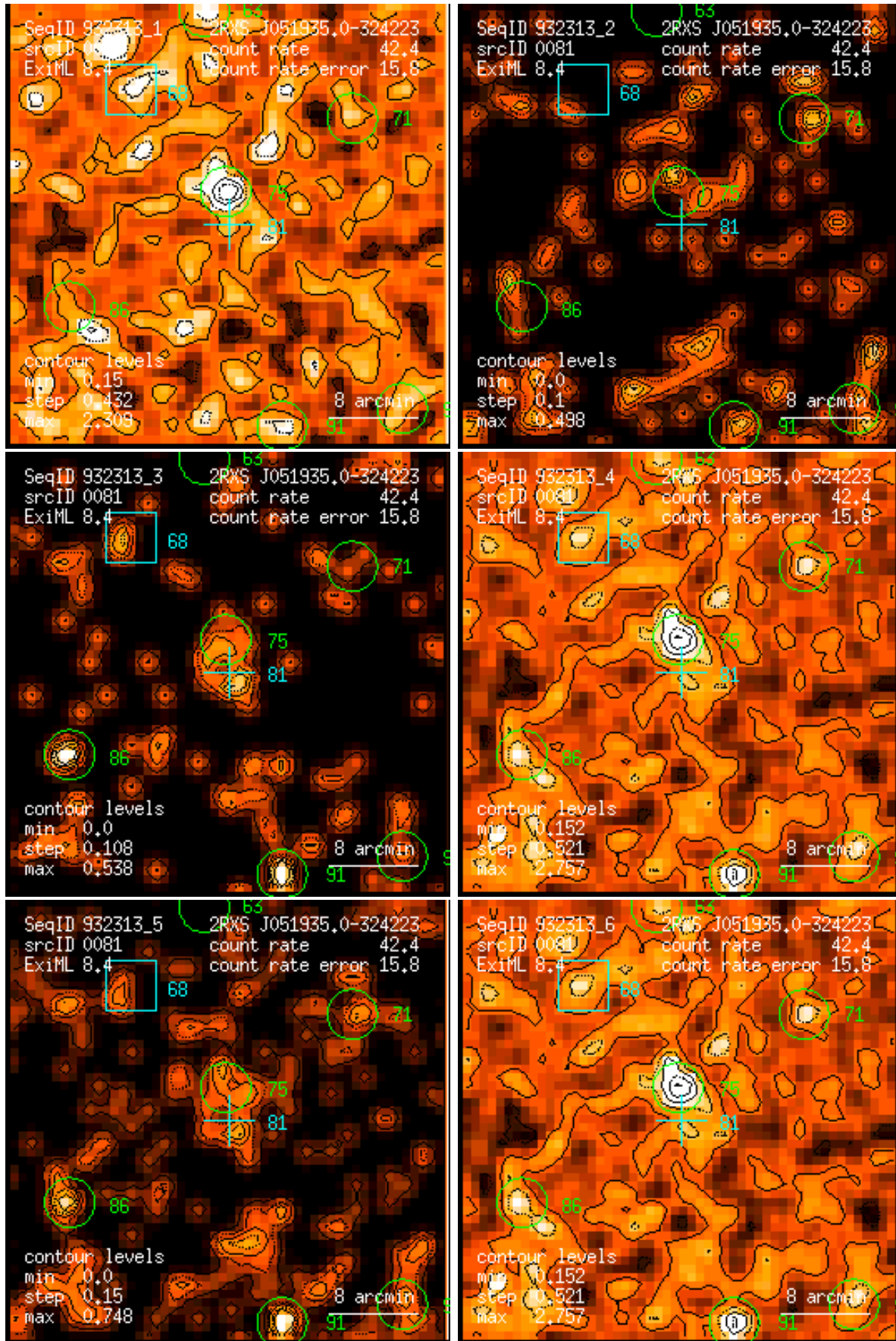
Figure 81: RASS 932313: detection 0081: band rate images, Gaussian filter: (1) PSPC channels 11 – 41, (2) 52 – 90, (3) 91 – 201, (4) 11 – 235, (5) 52 – 201, (6) 11 – 201. Broad band rates in counts/ks. Band rate contour levels in counts/ks/arcmin 2 .
