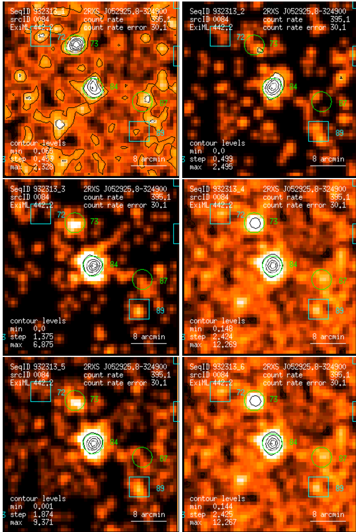
Figure 84: RASS 932313: detection 0084: band rate images, Gaussian filter: (1) PSPC channels 11 – 41, (2) 52 – 90, (3) 91 – 201, (4) 11 – 235, (5) 52 – 201, (6) 11 – 201. Broad band rates in counts/ks. Band rate contour levels in counts/ks/arcmin 2 .
