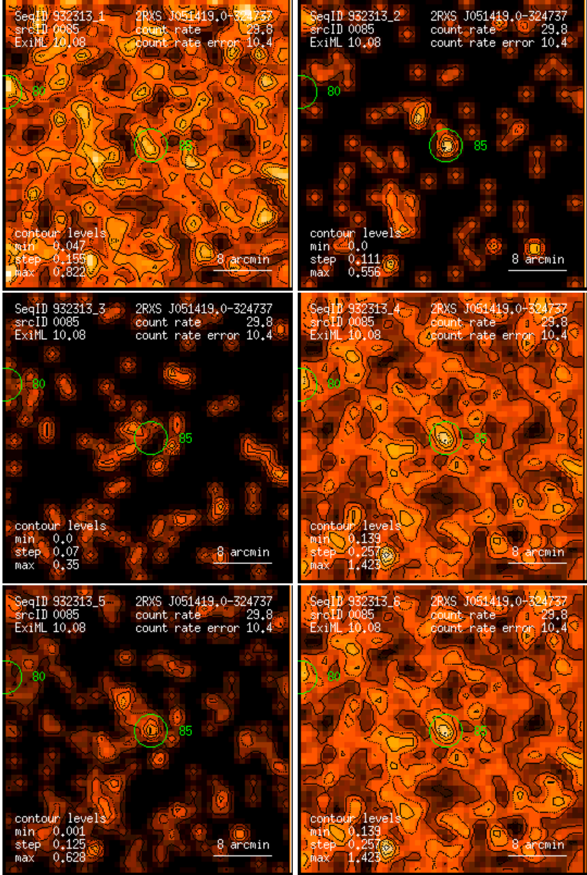
Figure 85: RASS 932313: detection 0085: band rate images, Gaussian filter: (1) PSPC channels 11 – 41, (2) 52 – 90, (3) 91 – 201, (4) 11 – 235, (5) 52 – 201, (6) 11 – 201. Broad band rates in counts/ks. Band rate contour levels in counts/ks/arcmin 2 .
