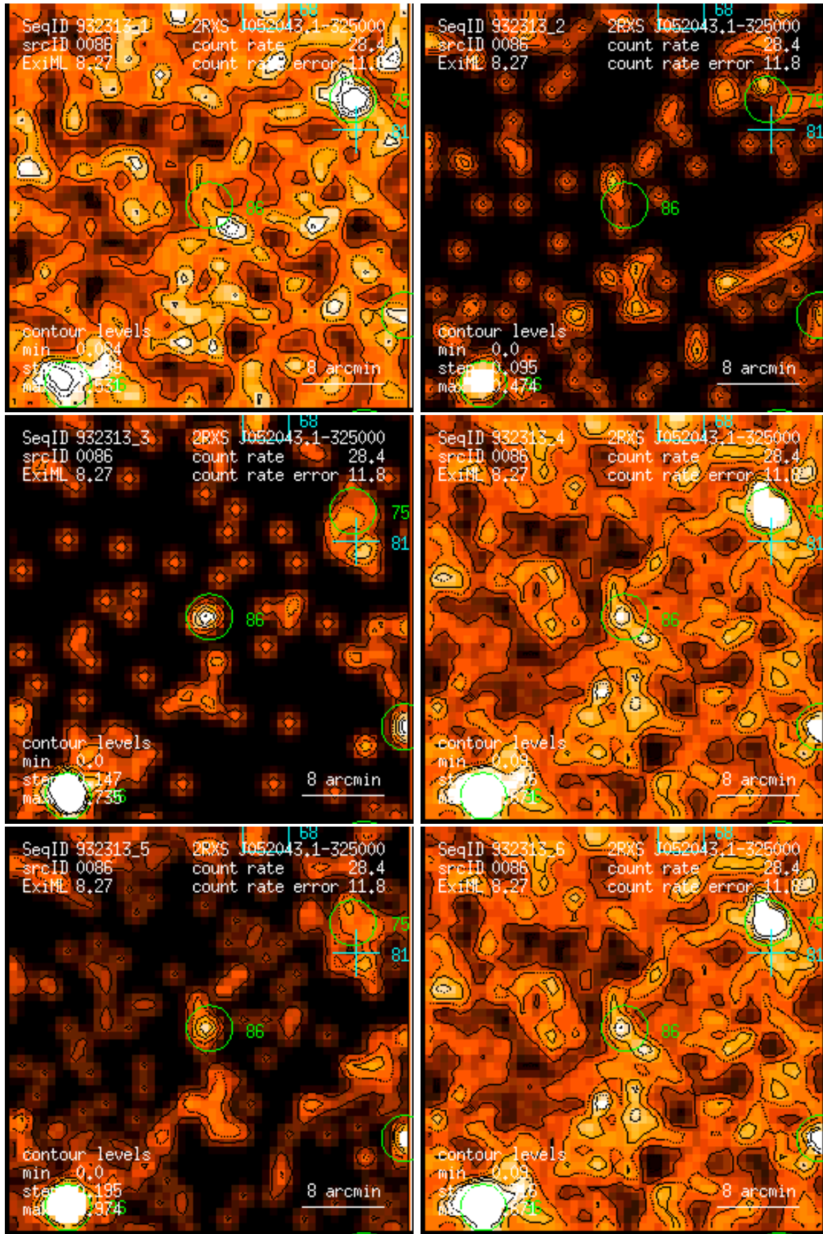
Figure 86: RASS 932313: detection 0086: band rate images, Gaussian filter: (1) PSPC channels 11 – 41, (2) 52 – 90, (3) 91 – 201, (4) 11 – 235, (5) 52 – 201, (6) 11 – 201. Broad band rates in counts/ks. Band rate contour levels in counts/ks/arcmin 2 .
