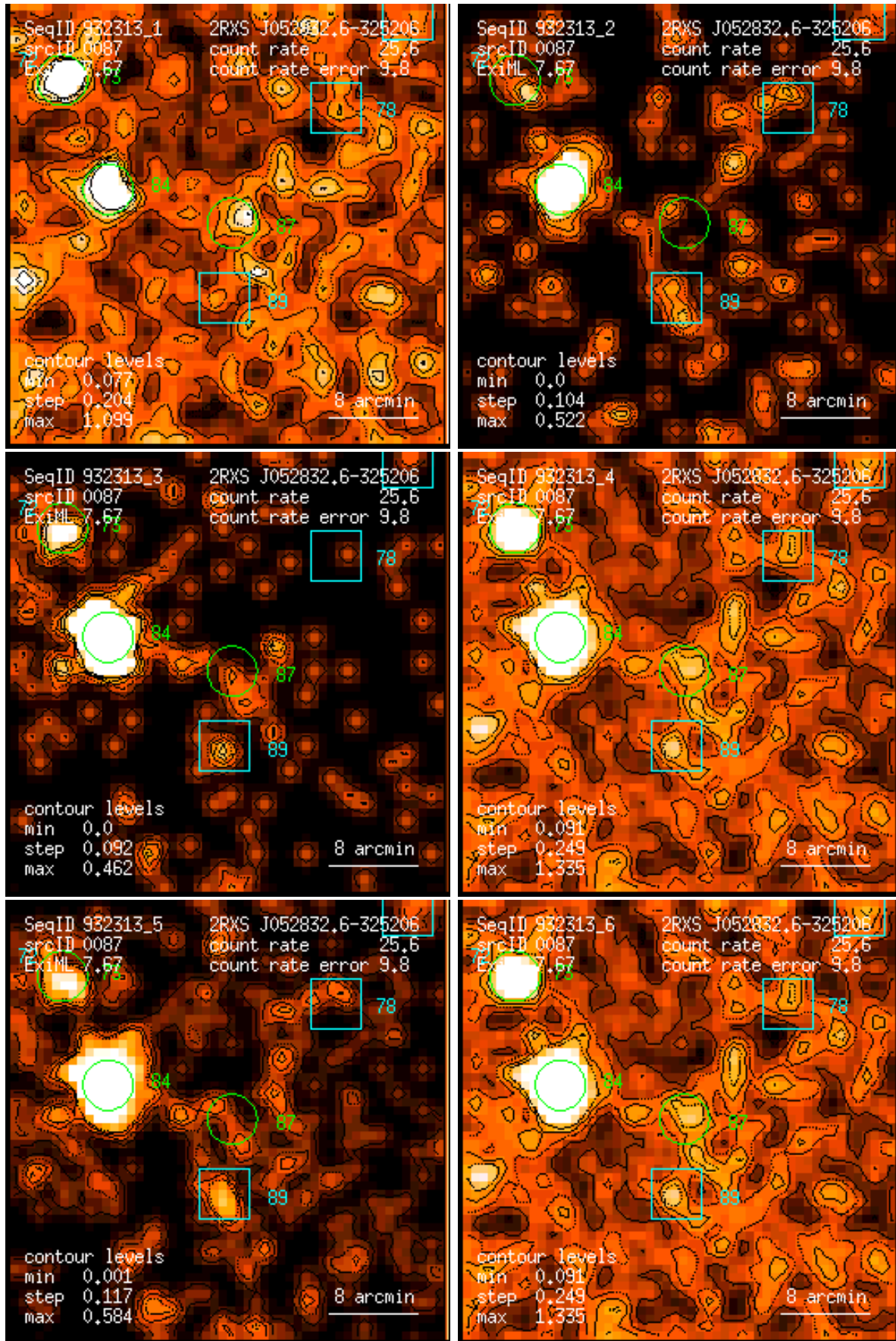
Figure 87: RASS 932313: detection 0087: band rate images, Gaussian filter: (1) PSPC channels 11 – 41, (2) 52 – 90, (3) 91 – 201, (4) 11 – 235, (5) 52 – 201, (6) 11 – 201. Broad band rates in counts/ks. Band rate contour levels in counts/ks/arcmin 2 .
