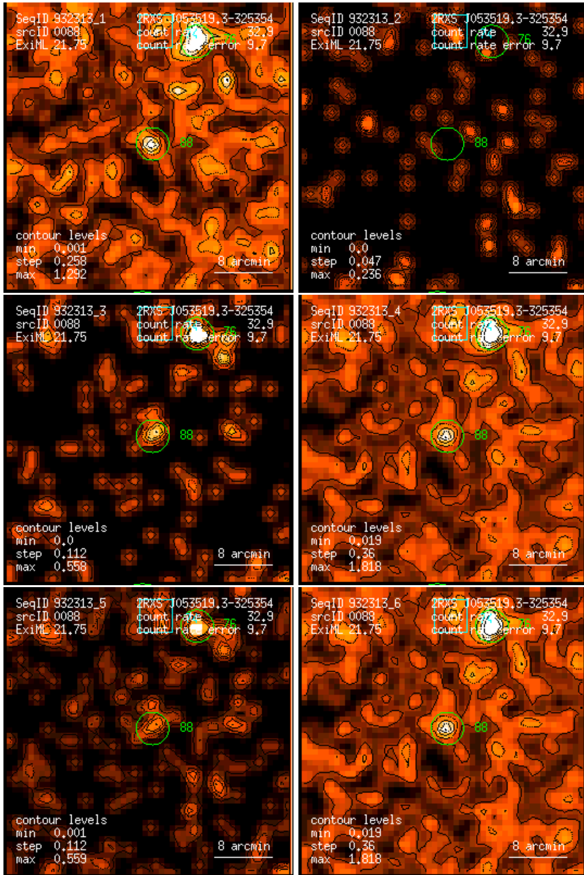
Figure 88: RASS 932313: detection 0088: band rate images, Gaussian filter: (1) PSPC channels 11 – 41, (2) 52 – 90, (3) 91 – 201, (4) 11 – 235, (5) 52 – 201, (6) 11 – 201. Broad band rates in counts/ks. Band rate contour levels in counts/ks/arcmin 2 .
