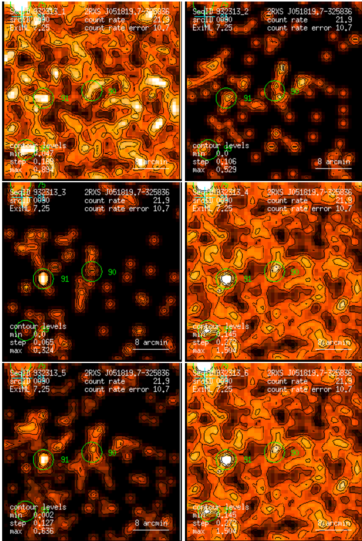
Figure 90: RASS 932313: detection 0090: band rate images, Gaussian filter: (1) PSPC channels 11 – 41, (2) 52 – 90, (3) 91 – 201, (4) 11 – 235, (5) 52 – 201, (6) 11 – 201. Broad band rates in counts/ks. Band rate contour levels in counts/ks/arcmin 2 .
