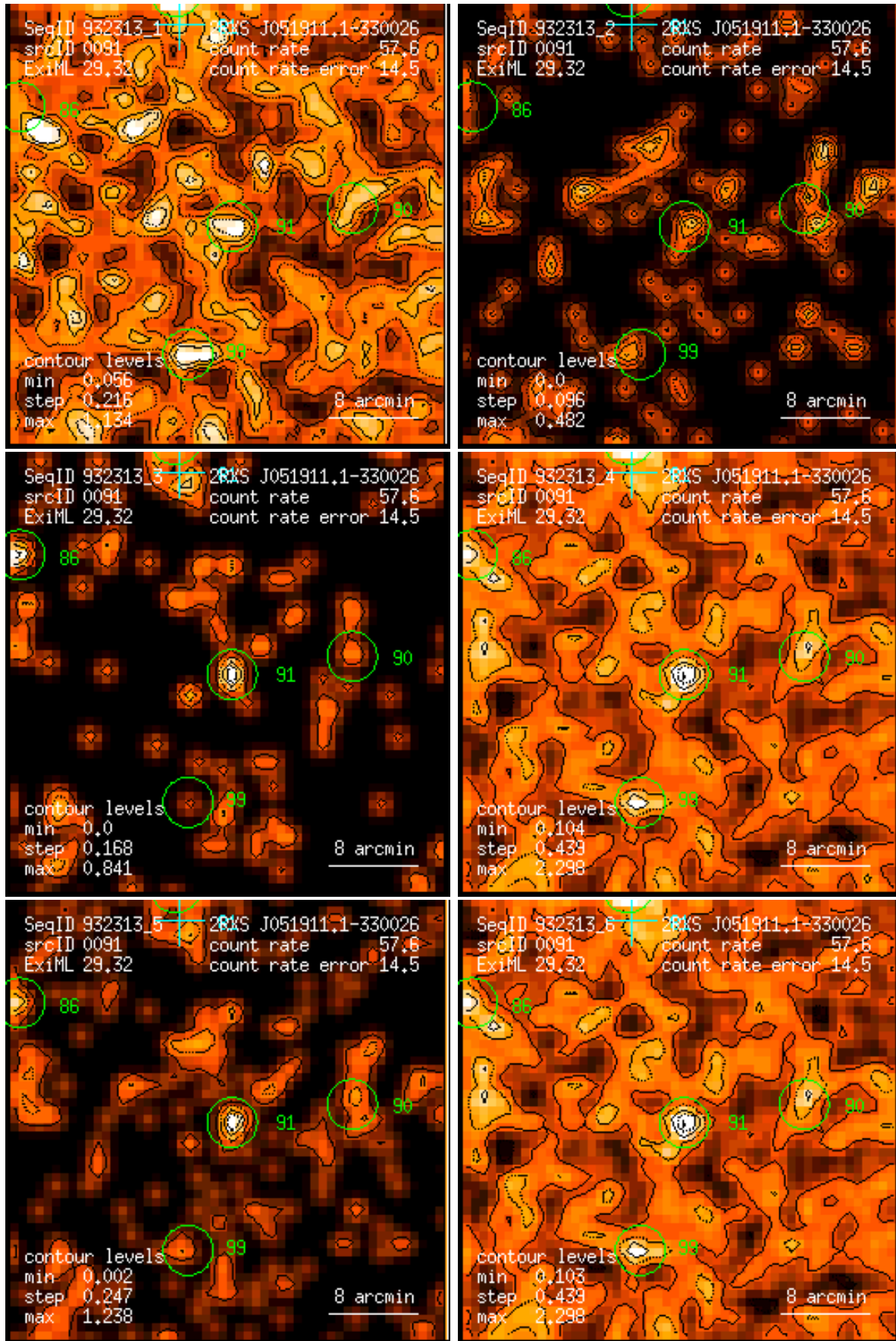
Figure 91: RASS 932313: detection 0091: band rate images, Gaussian filter: (1) PSPC channels 11 – 41, (2) 52 – 90, (3) 91 – 201, (4) 11 – 235, (5) 52 – 201, (6) 11 – 201. Broad band rates in counts/ks. Band rate contour levels in counts/ks/arcmin 2 .
