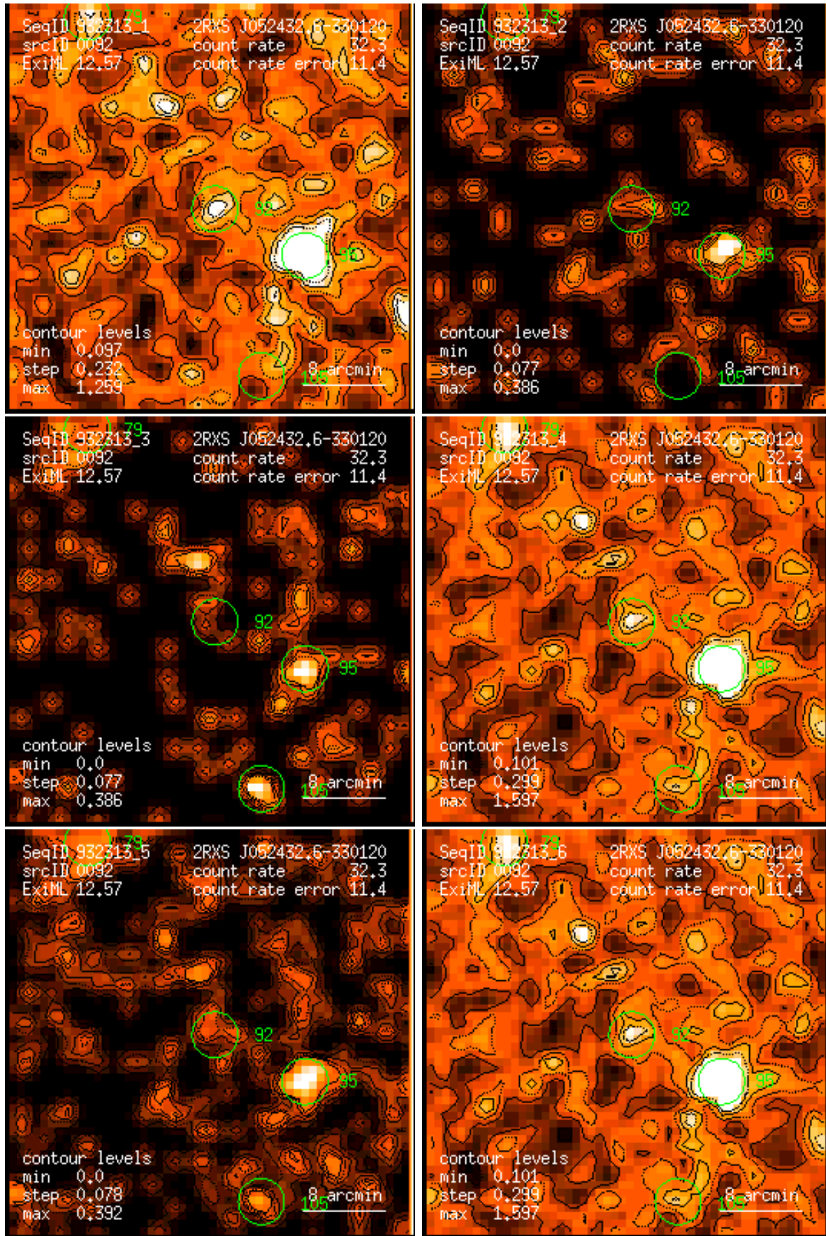
Figure 92: RASS 932313: detection 0092: band rate images, Gaussian filter: (1) PSPC channels 11 – 41, (2) 52 – 90, (3) 91 – 201, (4) 11 – 235, (5) 52 – 201, (6) 11 – 201. Broad band rates in counts/ks. Band rate contour levels in counts/ks/arcmin 2 .
