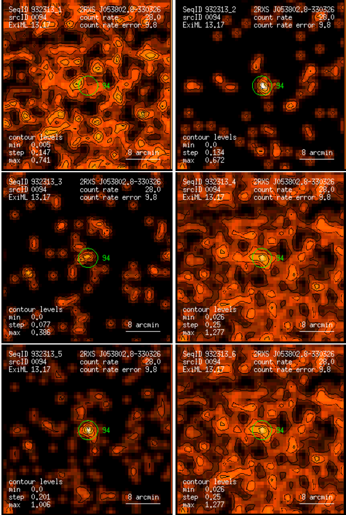
Figure 94: RASS 932313: detection 0094: band rate images, Gaussian filter: (1) PSPC channels 11 – 41, (2) 52 – 90, (3) 91 – 201, (4) 11 – 235, (5) 52 – 201, (6) 11 – 201. Broad band rates in counts/ks. Band rate contour levels in counts/ks/arcmin 2 .
